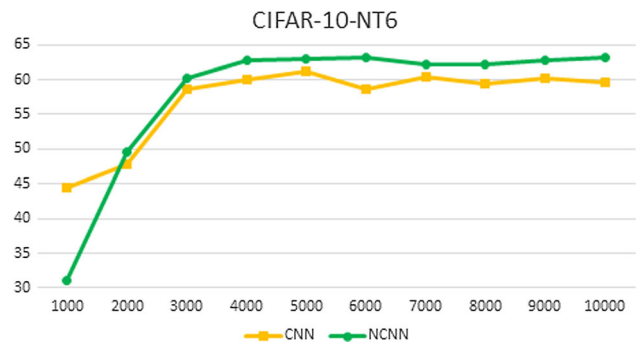
Fig. 21 Number of iteration versus accuracy in CIFAR-10-NT6 dataset
