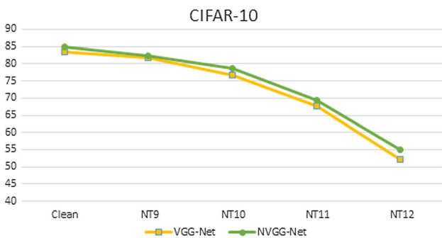
Fig. 16 NVGG-Net and VGG-Net accuracies with NT10 training data
