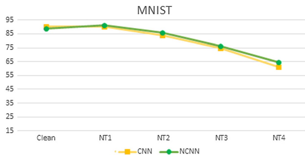
Fig. 6 NCNN and CNN accuracies with noisy training and noisy test data for MNIST
