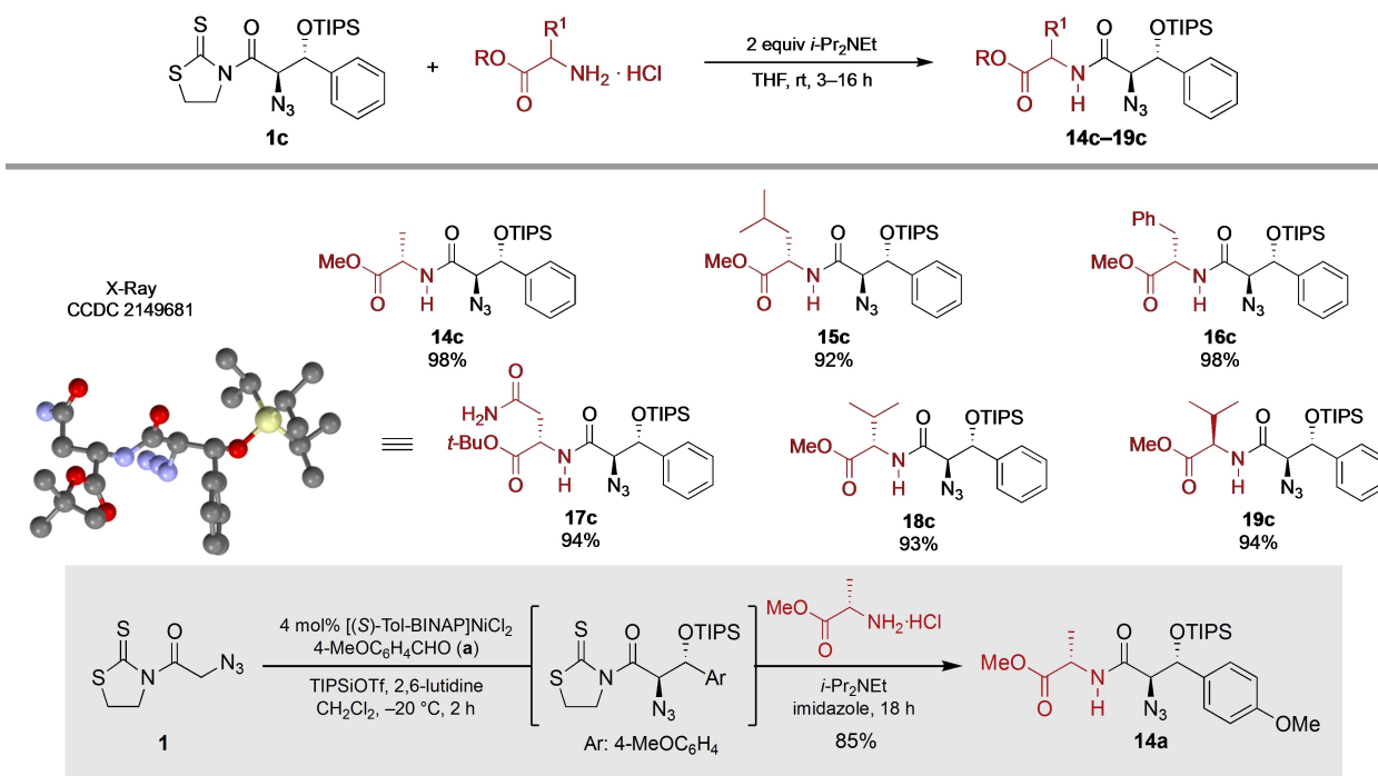
Scheme 4. Synthesis of dipeptides from \alpha -amino ester hydrochlorides.
