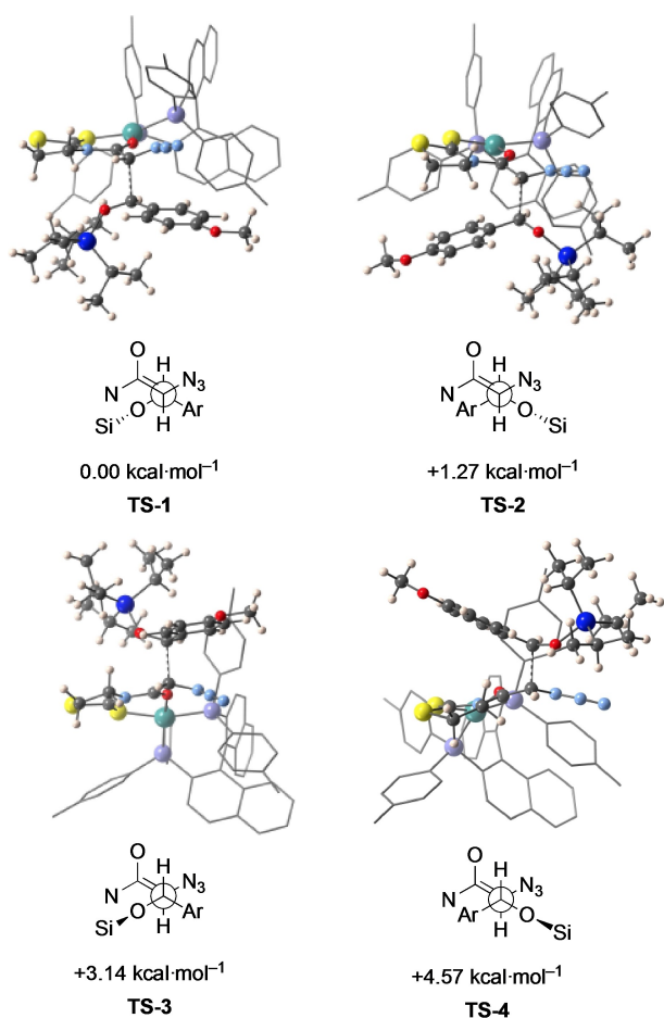
Figure 2. Accessible transition states for the reaction of 1 with a . The relative energies in \text{CH}_2\text{Cl}_2 are shown, taking the most stable one as reference.
