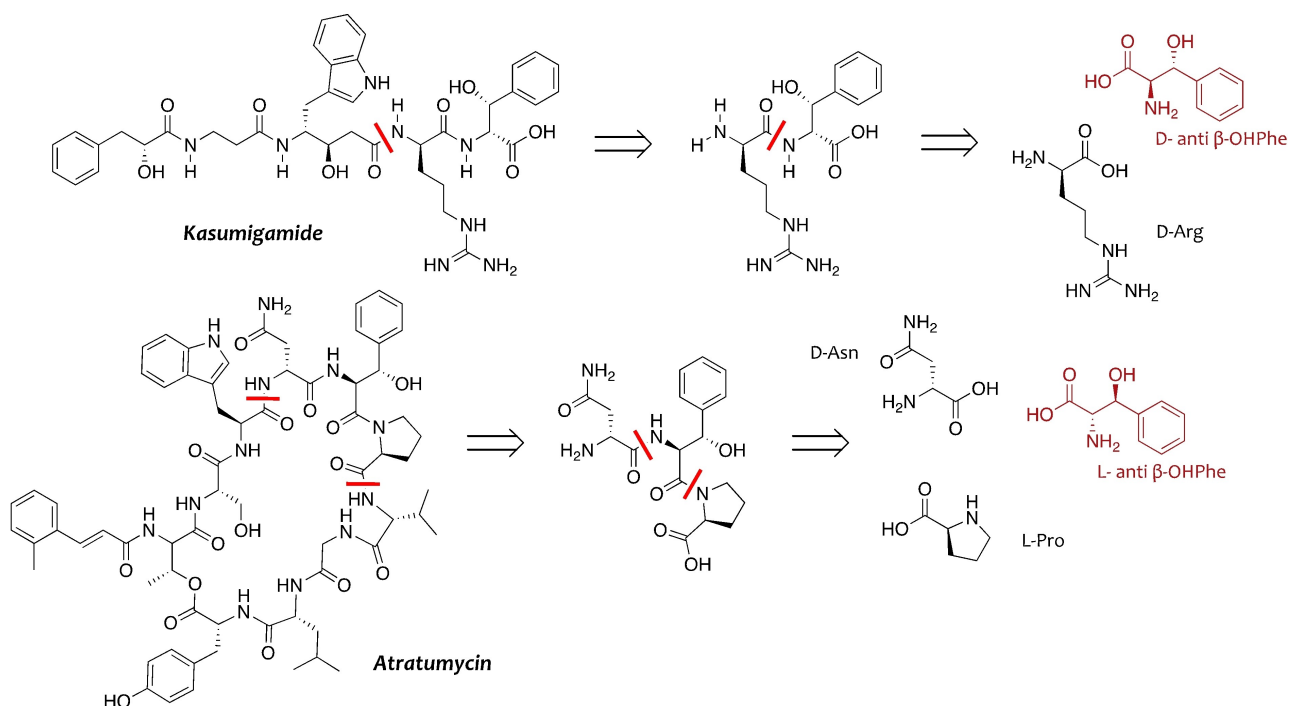
Scheme 6. Retrosynthetic analysis of kasumigamide and atratumycin.
