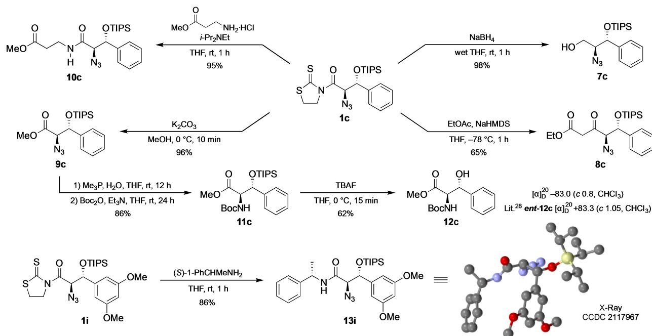
Scheme 3. Synthesis of enantiomerically pure derivatives.
