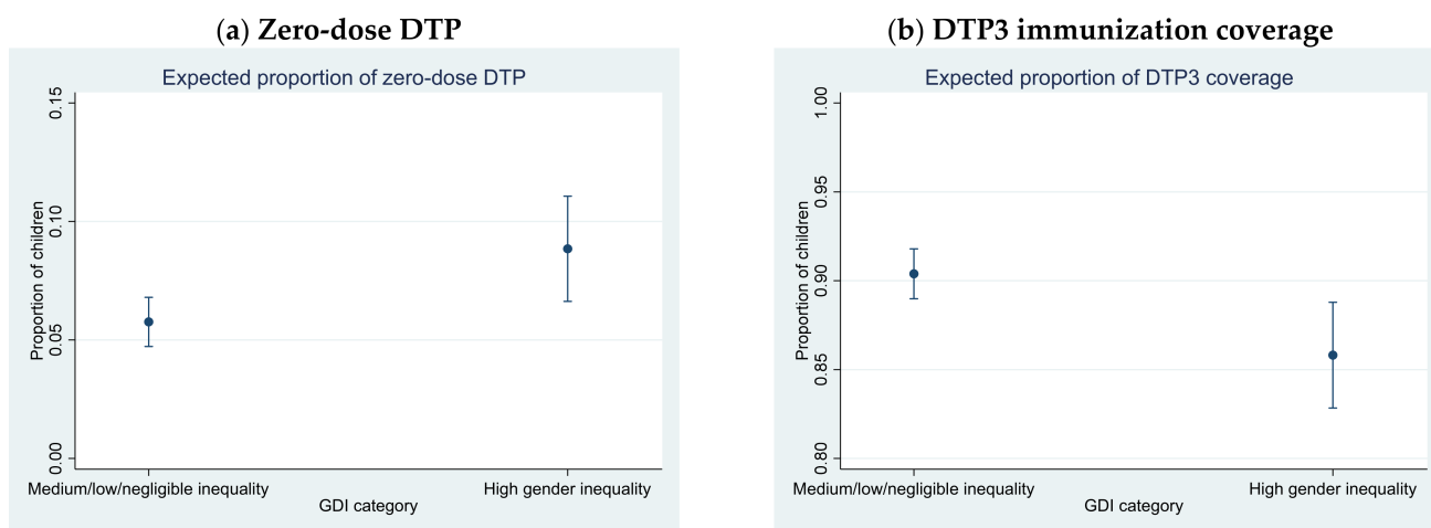
Figure 1. Adjusted proportions of (a) zero-dose DPT and (b) DTP3 immunization coverage for categories of GDI, 164 countries (1 country did not have available data for this model), 2010–2019. Note: The estimated proportions are adjusted for annual population growth and age structure (measured as the percentage of the population under 15 years of age), percentage of urban population, and the three individual dimensional indices of the HDI (health index, education index, and GNI index).
