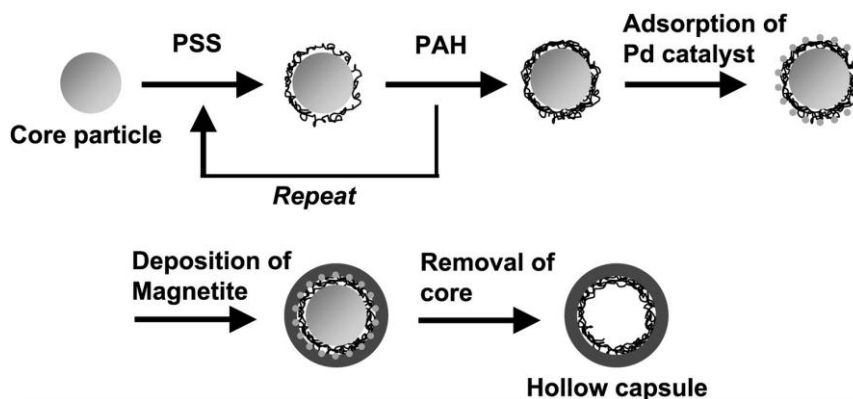
Figure 3. Formation of \text{Fe}_3\text{O}_4 /Pd/polyelectrolyte hybrid capsules by layer-by-layer deposition. Reprinted with permission from [29]. Copyright 2010, Elsevier.
