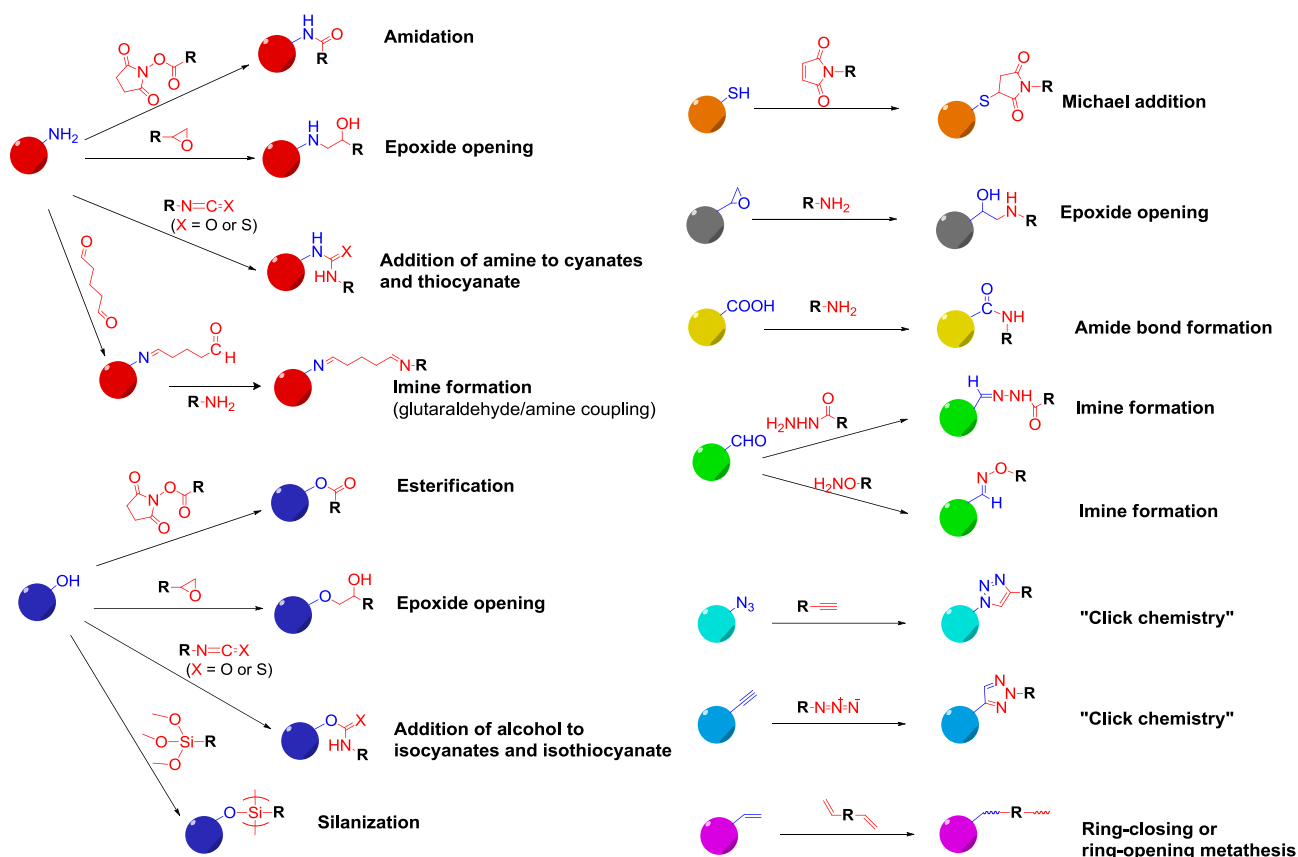
Figure 4. Main strategies for covalent post-functionalization of nanoparticles. Reproduced with permission from [20], partially based on Erathodiyl and Ying [37]. Copyright 2013, Eureka Science Ltd.
