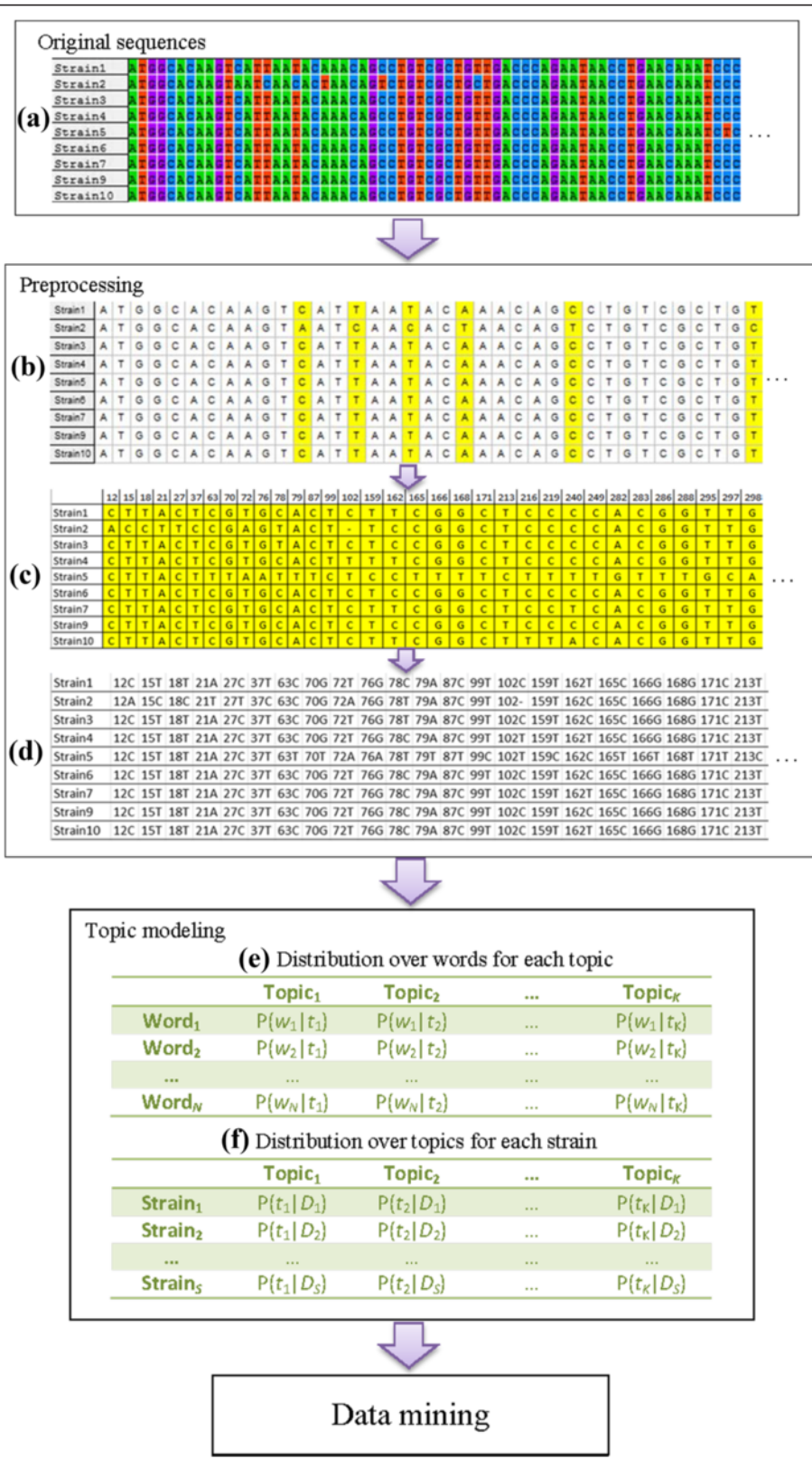
Fig. 1 Flowchart of the proposed procedure
