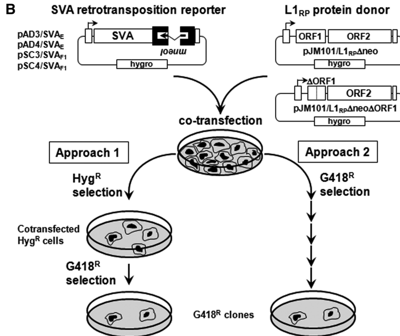
Figure 1. Rationale of the SVA trans -mobilization assay. (A) Schematic representation of SVA retrotransposition reporter plasmids, and pseudogene-formation control construct pCEPneo. SVA reporter elements in pAD3/SVA E , pAD4/SVA E , pSC3/SVA F1 and pSC4/SVA F1 and the processed pseudogene formation cassette in pCEPneo were each tagged with the indicator gene mneol , and set under transcriptional control of the human CMV promoter (CMV P ). Splice donor (SD) and splice acceptor (SA) sites of the oppositely oriented \gamma -globin intron are indicated. mneol is flanked by a heterologous promoter (P') and a polyadenylation signal (A'). Transcripts originating from CMV P driving SVA mneol or CEP mneol transcription can splice the intron, but contain an antisense copy of the neo gene. G418 resistant (G418 R ) colonies arise only if this transcript is reverse transcribed, integrated into chromosomal DNA, and expressed from its own promoter P'. Each SVA reporter element was inserted between CMV P and the mneol cassette. pAD4/SVA E differs from pAD3/SVA E in the deletion of the initial 498 nt of the SVA 5'-end covering (CCCTCT) n - and Alu -like region. pSC4/SVA F1 varies from pSC3/SVA F1 in the insertion of the 389-bp AluSp element fused to the A 14 TTTA 26 stretch between
