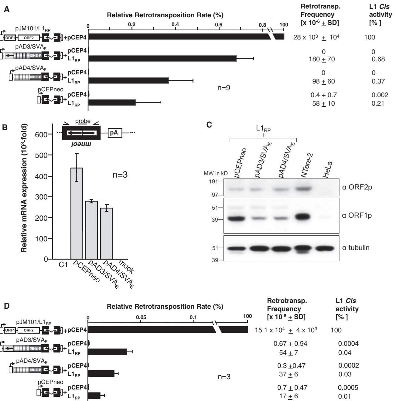
Figure 2. Trans-mobilization of mneoI -tagged SVA E reporter elements. (A) SVA E retrotransposition reporter assay after hygromycin selection for the presence of expression plasmids. SVA E reporter plasmids pAD3/SVA E , pAD4/SVA E , or pCEPneo were cotransfected with the L1 protein donor pJM101/L1 RP Δneo (L1 RP ) or the empty vector pCEP4. After hyg R selection, G418 R selection for retrotransposition events followed and retrotransposition rates were determined by counting G418 R HeLa colonies. Each cotransfection experiment and subsequent retrotransposition reporter assay was carried out three times in triplicates. Retrotransposition frequencies per 10 6 cells are listed and relative retrotransposition rates are indicated as bar diagram. Cis retrotransposition rate of the L1 reporter element pJM101/L1 RP was set as 100%. Each bar depicts the arithmetic mean ± SD of the relative retrotransposition rates obtained from nine individual cotransfection experiments ( n = 9). (B) qRT-PCR analyses to quantify the relative amounts of spliced transcripts expressed from retrotransposition reporter cassettes. Total RNA was isolated 48 h after cotransfection of pCEPneo, pAD3/SVA E , and pAD4/SVA E with the L1 protein donor plasmid pJM101/L1 RP Δneo. The used primer/probe combination (see ‘Materials and Methods’ section) is specific for the spliced mneoI -cassette (black box with arrow). Relative amounts of mRNA expression refer to the signal obtained from total RNA of untransfected HeLa cells which was set as 1 (C1); Total RNA from mock-transfected HeLa cells served as negative control. (C) Immunoblot analysis of L1 protein expression in HeLa cells after cotransfection of the L1 protein donor (L1 RP ) with retrotransposition reporter plasmids pAD3/SVA E , pAD4/SVA E and pCEPneo. Whole-cell lysates were prepared 14 days after cotransfection upon completion of hygromycin selection and subjected to immunoblot analysis using antibodies against either L1 ORF1p (αORF1p) or L1 ORF2p (αORF2p). An amount of 20 μg of whole-cell extracts were loaded per lane. α-tubulin protein levels (~50 kDa) were analyzed as loading control. Lysates from untransfected HeLa cells and from the germ cell tumor cell line Ntera-2 served as negative and positive control for L1 protein detection, respectively. (D) SVA E trans-mobilization assay after transient cotransfection of expression plasmids. pAD3/SVA E , pAD4/SVA E or pCEPneo were transiently cotransfected with pJM101/L1 RP Δneo (L1 RP ) or pCEP4 into HeLa cells. Two days later, cells were G418-selected for de novo retrotransposition events for 14 days. G418 R HeLa colonies were Giemsa-stained and counted. Each cotransfection experiment was done in quadruplicate. Subsequent retrotransposition reporter assays were performed in triplicate. Retrotransposition frequencies per 10 6 cells are listed and relative retrotransposition rates are indicated as bar diagram. Cis retrotransposition rate of L1 reporter element pJM101/L1 RP was set as 100%. Each bar depicts the arithmetic mean ± SD of the relative retrotransposition rates obtained from three individual cotransfection experiments ( n = 3).
