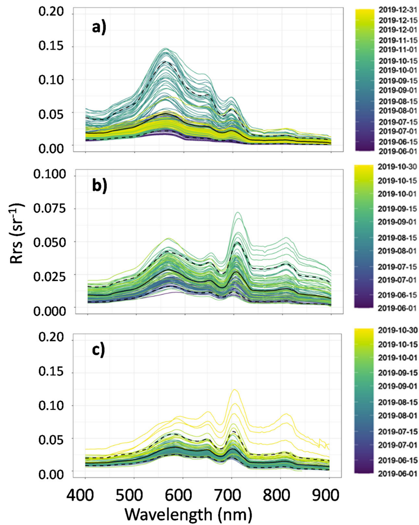
Figure 4. Daily averages of Remote sensing reflectances (Rrs) for the period of measurement in Lake Trasimeno from 1 June to 31 December 2019 (a), Curonian Lagoon (b), and Lake Vörtsjärv (c) from 1 June to 31 October 2019. Black continuous line is the Rrs mean value computed over the entire period and black dotted lines are the relative 5th and 95th percentiles.
