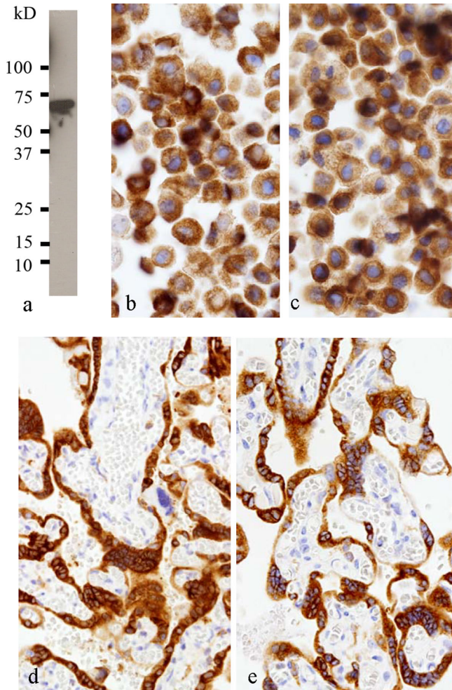
Fig. 1. Characterization of the anti-IMP3 antibody. Western blotting of A549 cell lysate using an anti-IMP3 antibody identifies a single band corresponding to the predicted molecular weight of approximately 70 kDa (a). Immunohistochemical staining of IMP3 in A549 cells and placental tissue fixed for 1 day (b, d) and 14 days (c, e). A549 cells (b, c) and syncytiotrophoblasts in placental villi (d, e) show diffuse and intense cytoplasmic staining of IMP3. (b)–(e): IMP3 immunohistochemistry.
