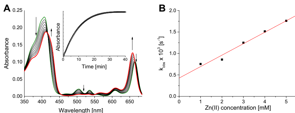
Fig. 1 Changes in the absorption spectrum accompanying the reaction of Pheoa (green line) with \text{Zn}(\text{II}) chloride in methanol (a). Red line the spectrum of the final product, \text{Zn-Pheoa} . Note isosbestic points near 410, 450, 550 and 660 nm. Inset: the kinetic trace recorded at 655 nm and 298 K for a 2000-fold excess of \text{Zn}(\text{II}) . Dependence of the k_{\text{obs}} values on [\text{ZnCl}_2] determined for the reaction at 298 K (b)
