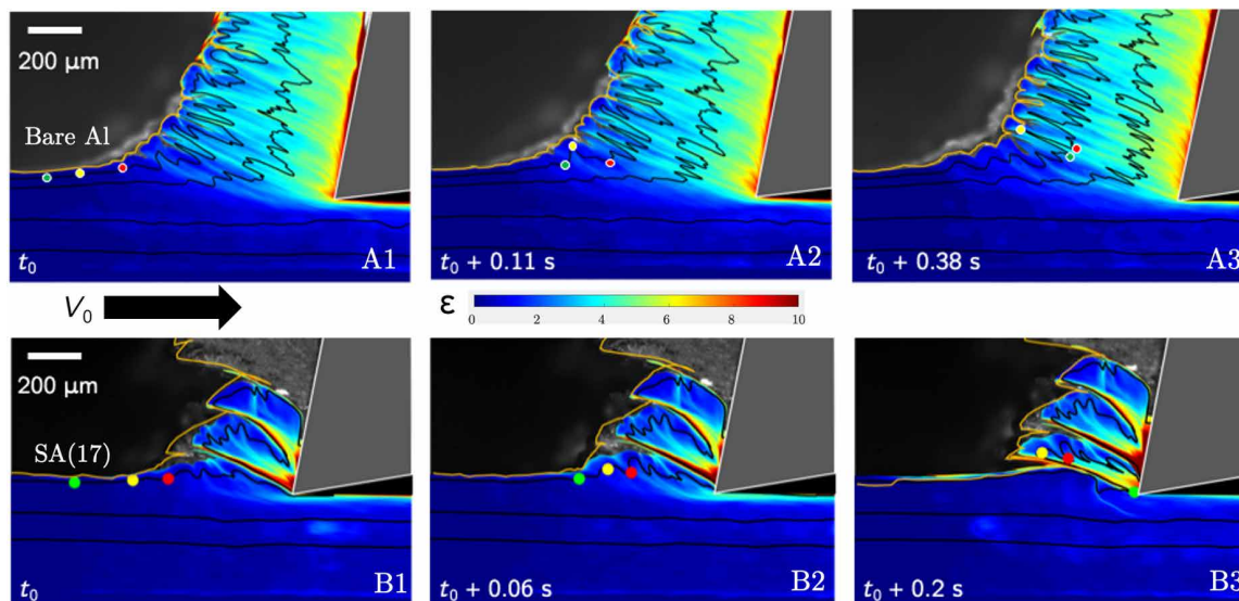
Fig. 3. High-speed imaging of (contrasting) plastic flow modes reveals origin of MC effect. Select images, with strain-field (background color) and streaklines superimposed, show development of flow with [bottom row, SA(17)] and without (top row, bare Al) long-chain SAMs. (Top) With bare Al workpiece, the shearing results in sinuous flow with thick-chip, wavy streaklines, and heterogeneous straining. Flow development is tracked via green, yellow, and red points (initially collinear, frame A1). A bump forms on workpiece surface ahead of chip in frame A2. The bump grows in amplitude, rotates, and shears to form a fold in frame A3. The final chip is a stack of folds, with fold interfaces resembling notches. (Bottom) With a long-chain SAM [SA(17)], the shearing results in segmented flow—typical of MC effect. Movement of green, yellow, and red points in frames B1 and B2 is similar to frames A1 and A2 (top row). However, between frames B2 and B3, a crack starts from workpiece surface and propagates toward wedge tip, causing a large separation between yellow and green points. This cracking, which arrests the sinuous flow in its incipient stage, is recurrent and results in segmented flow.
