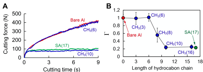
Fig. 2. Characterizing MC effect using cutting force. (A) Comparison of force with and without SAM films. A large force decrease (~85%), typical of the MC effect, is seen with the long-chain SAMs [CH 3 (10) and SA(17)]. (B) Plot of the ratio ( \Gamma )—maximum cutting force with a specific SAM film to the maximum cutting force without any film (bare)—as a function of chain length. A sharp decrease in \Gamma from 1 to ~0.15 occurs as chain length increases from 6 to 10, indicating the importance of chain length in controlling the MC effect.
