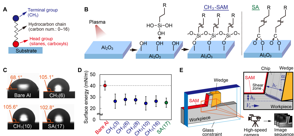
Fig. 1. Using SAMs to probe MC effect. (A) Schematic of a molecule adsorbed on metal surface showing head and terminal groups, and hydrocarbon chain. (B) Procedure to deposit SAMs: For the silane head molecules, workpiece is first plasma-treated to increase hydroxyl group density at surface and then immersed in ethanol solution containing the molecule. For the stearic acid SAM, workpiece is directly immersed in ethanol solution containing stearic acid. (C) SAM-deposited workpiece surfaces characterized by contact angle measurement. (D) Surface energy obtained from the contact angle using the Owens-Wendt theory (34). Because surface energy is determined purely by terminal group, all the SAMs show a uniform reduction of \sim 37\% in this energy. (E) Model 2D experimental (simple shear) configuration used to explore MC effect with SAM films (red). A high-speed camera, coupled to an optical microscope, is used to image material flow and characterize plastic flow field.
