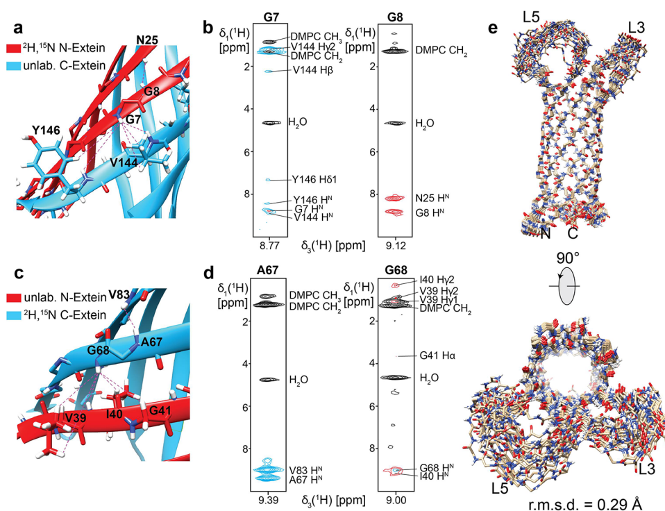
Figure 5. Segmental isotope labeling of membrane proteins facilitates NMR structure determination. (a) Structural interface between ^2\text{H}, ^{15}\text{N} -labeled OmpX-N-extein and unlabeled OmpX-C-extein with observed NOE distance restraints (shown in (b)) within the labeled or to the unlabeled part. (c) and (d), same as in (a) and (b) but with an inverse isotope labeling pattern, i.e., ^2\text{H}, ^{15}\text{N} -labeled OmpX-C-extein and unlabeled OmpX-N-extein. (e) 2D NMR spectra of OmpX in lipid nanodiscs, showing a root mean square deviation (rmsd) of backbone atoms in ordered secondary structure elements of 0.29 Å. The assignment of NOE contacts was facilitated by the lower complexity and signal overlap in the individual spectra.
