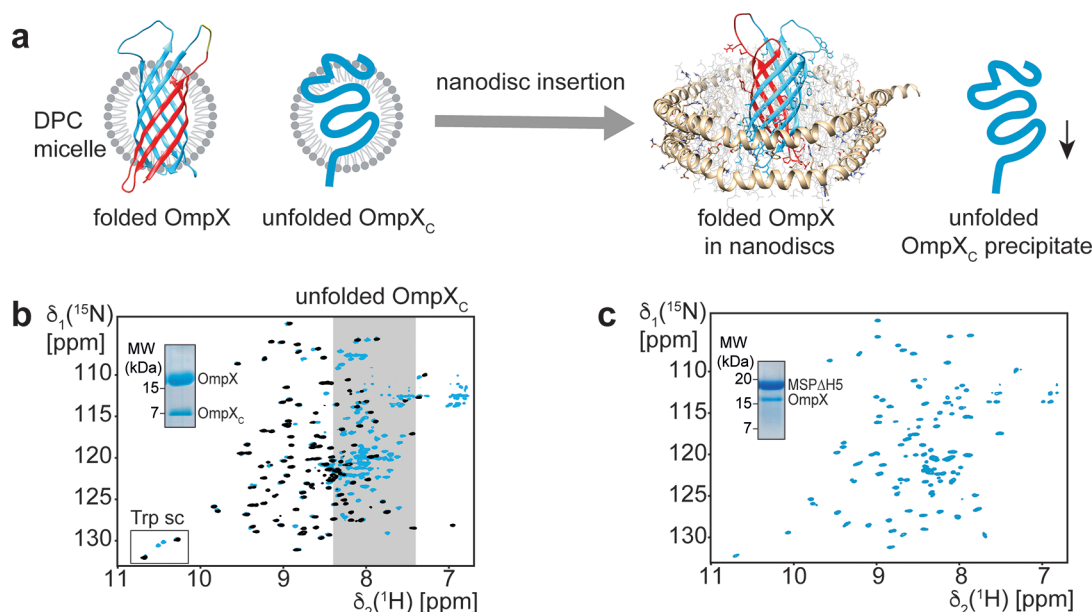
Figure 3. Removal of ligation side products by insertion into lipid nanodiscs. (a) After intein splicing and refolding, properly folded full-length and a misfolded OmpX C fragment are copurifying in DPC detergent micelles, giving rise to a 2D- ^{15}\text{N} , ^1\text{H} -TROSY spectrum containing signals of both species (blue spectrum in panel b). The black spectrum in (b) is a reference with folded U - ^{2}\text{H} , ^{15}\text{N} -labeled OmpX in DPC micelles. Insertion into lipid nanodiscs selects for the properly folded species and efficiently removes the OmpX C fragment, indicated by SDS-PAGE and a 2D- ^{15}\text{N} , ^1\text{H} -TROSY spectrum lacking signals in the unfolded region (c). NMR spectra were recorded at 318 K and at 950 MHz ^1\text{H} frequency with a sample where the C-extein of OmpX (Figure 1b) is labeled with ^2\text{H} and ^{15}\text{N} (blue spectra). The N-extein is unlabeled and not visible in NMR. Trp sc: tryptophane NH \epsilon side chain signals.
