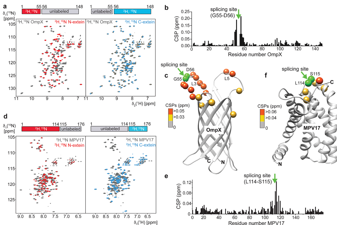
Figure 4. 2D-NMR analysis of the segmentally isotope-labeled integral membrane proteins OmpX and MPV17. (a) 2D- ^{15}\text{N} , ^1\text{H} -TROSY spectra of uniformly labeled OmpX (gray) and segmentally labeled OmpX (red and blue). (b) Chemical shift perturbations (CSPs) within OmpX calculated from the spectra shown in (a). (c) CSPs mapped onto the structure of OmpX (2m06.pdb 4 ). The splicing site is indicated by the two green spheres. (d–f) Same as in (a–c) but with segmentally isotope labeled MPV17 in DPC micelles. The structural model of MPV17 was obtained with AlphaFold. 20
