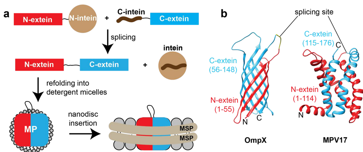
Figure 1. Intein-mediated protein trans-splicing for segmental isotope labeling of membrane proteins for NMR studies. (a) Strategy to obtain properly folded membrane proteins in detergent micelles and nanodiscs by protein trans-splicing. (b) Prototype membrane proteins OmpX (2m06.pdb 4 ) and MPV17 (AlphaFold 20 model) with a \beta -barrel and \alpha -helical topology, respectively. The N- and C-exteins and the splicing sites are indicated. MSP, membrane scaffold protein; MP, membrane protein.
