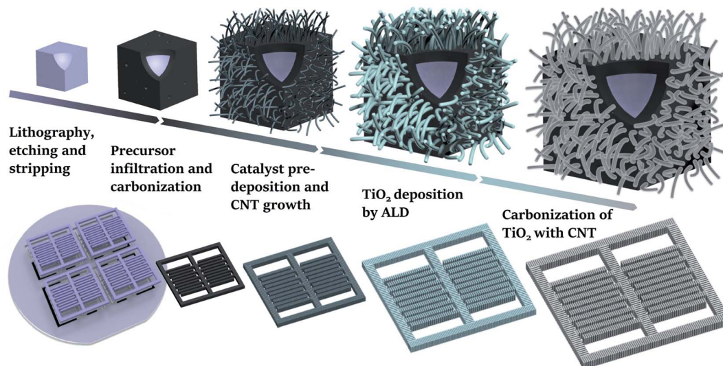
Fig. 1 Schematic illustration of the fabrication process of the 3D interdigital Si/C/CNT@TiC MSC including bulk micromachining technology, photoresist pyrolysis, CVD, ALD and in situ thermal reduction.
