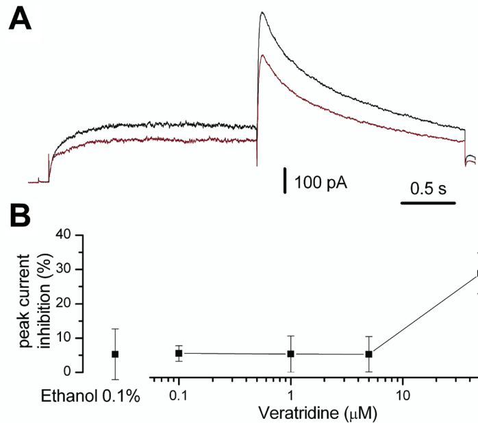
Figure 5. Effects of veratridine on hERG channels. A. Current traces in control conditions (upper) and during application of veratridine 50 \mu\text{M} (lower trace). B. Percentages of peak hERG current inhibition by different concentrations of veratridine and control ethanol 0.1% vehicle. Error bars represent SD. Number of experiments: control ( n = 6 ), veratridine 0.1 \mu\text{M} ( n = 10 ), 1 \mu\text{M} ( n = 5 ), 5 \mu\text{M} ( n = 7 ), 50 \mu\text{M} ( n = 10 ).
