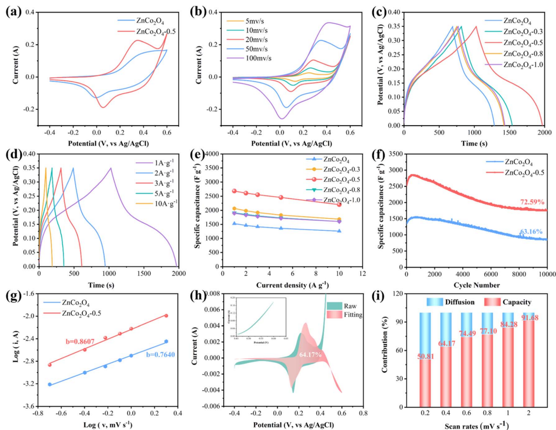
Fig. 4 (a) CV curves of \text{ZnCo}_2\text{O}_4 and \text{ZnCo}_2\text{O}_4\text{-}0.5 nanoclusters at the scan rate of 50 \text{ mV s}^{-1} . (b) CV curves at different scan rates of \text{ZnCo}_2\text{O}_4\text{-}0.5 nanoclusters. (c) GCD curves of \text{ZnCo}_2\text{O}_4 and OV- \text{ZnCo}_2\text{O}_4 (with different \text{NaBH}_4 concentrations) at the current density of 1 \text{ A g}^{-1} . (d) GCD curves at different current densities of \text{ZnCo}_2\text{O}_4\text{-}0.5 nanoclusters. (e) Specific capacitances of \text{ZnCo}_2\text{O}_4 and OV- \text{ZnCo}_2\text{O}_4 (with different \text{NaBH}_4 concentrations) at different current densities. (f) Cycling stability at 3 \text{ A g}^{-1} of pristine \text{ZnCo}_2\text{O}_4 and \text{ZnCo}_2\text{O}_4\text{-}0.5 nanoclusters. (g) Linear relationship of \log(i) and \log(v) for pristine \text{ZnCo}_2\text{O}_4 and \text{ZnCo}_2\text{O}_4\text{-}0.5 nanoclusters. (h) Separation of capacitance (red) controlled currents of \text{ZnCo}_2\text{O}_4\text{-}0.5 nanoclusters at 0.4 \text{ mV s}^{-1} . (i) Contributions of capacitance-controlled (red region) and diffusion-controlled (blue region) processes at different scan rates of \text{ZnCo}_2\text{O}_4\text{-}0.5 nanoclusters.
