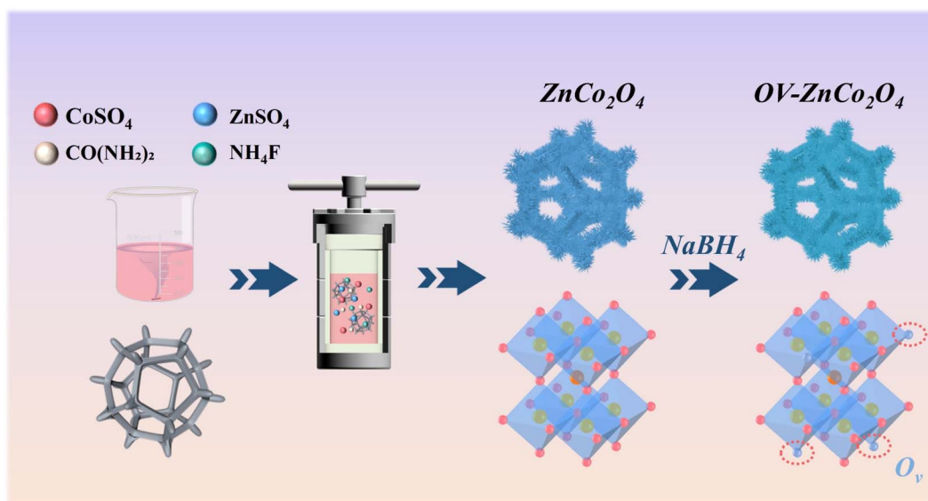
Scheme 1 The synthetic illustration of pristine \text{ZnCo}_2\text{O}_4 and \text{ZnCo}_2\text{O}_4\text{-}0.5 nanoclusters.
