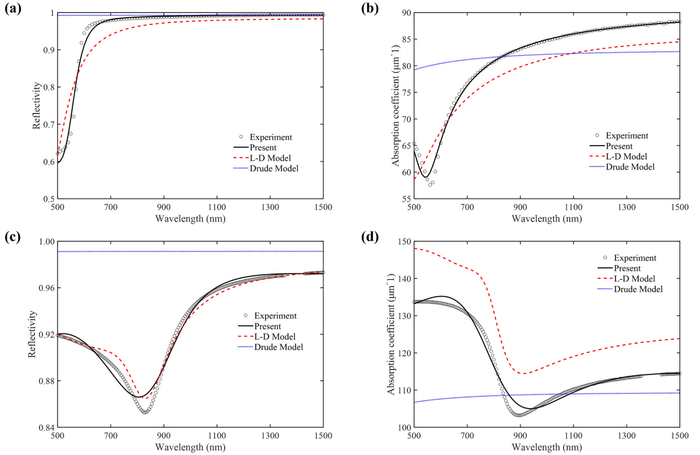
Fig. 2. (a) Reflectivity at room temperature versus wavelength calculated by different models for copper nanofilms (b) Absorption coefficient at room temperature versus wavelength calculated by different models for copper nanofilms (c) Reflectivity at room temperature versus wavelength calculated by different models for AlCu nanofilms (d) Absorption coefficient at room temperature versus wavelength calculated by different models for AlCu nanofilms.
