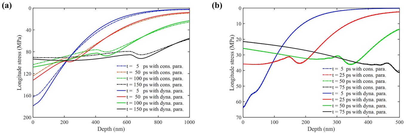
Fig. 6. (a) Profile of longitudinal stress in the copper nanofilm at various times calculated by different models (b) Profile of longitudinal stress in the AlCu nanofilm at various times calculated by different models.
