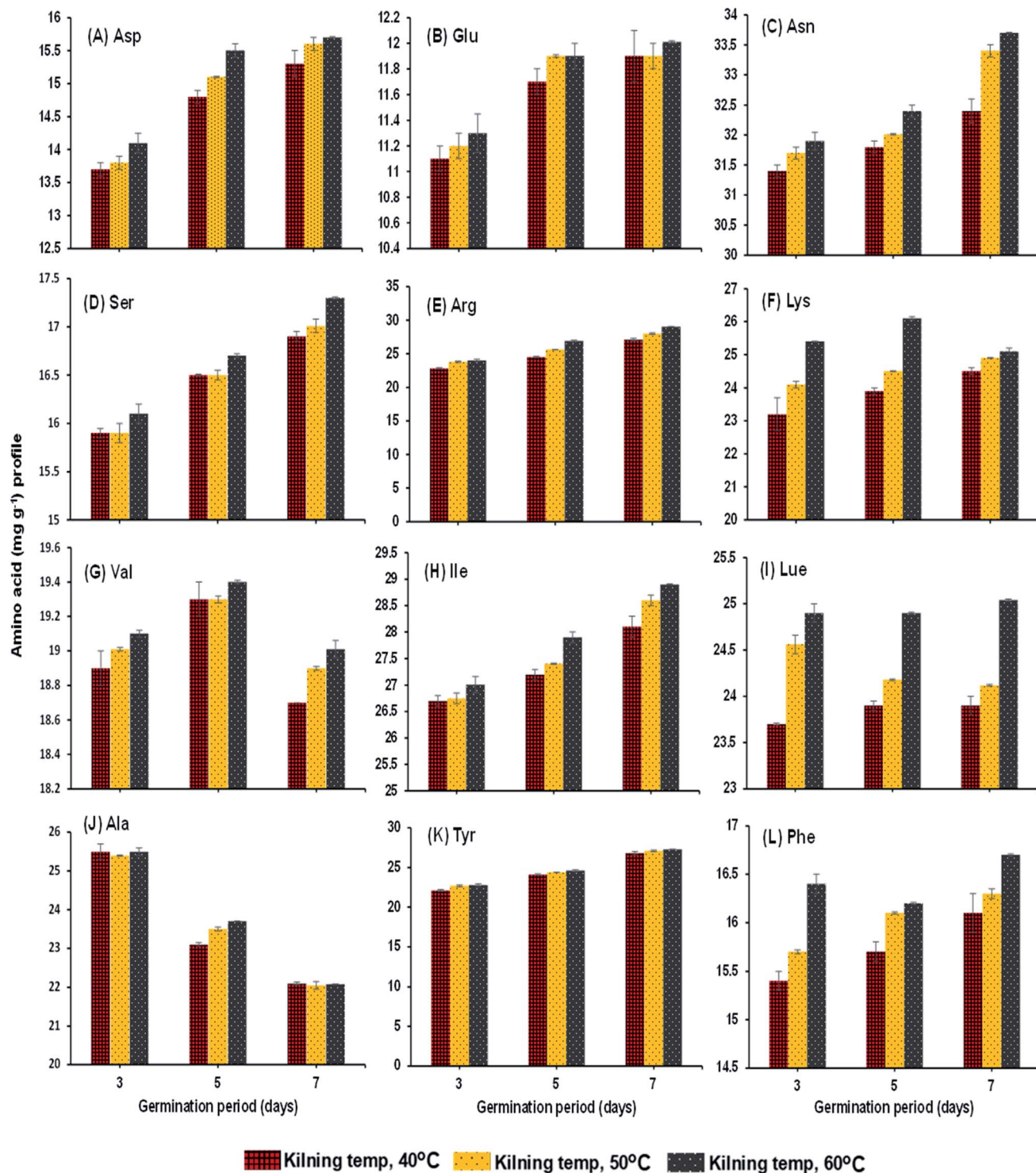
Fig. 4 Amino acid profile of malted HomChaiya rice granules at different germination times when kilned at different temperatures.
