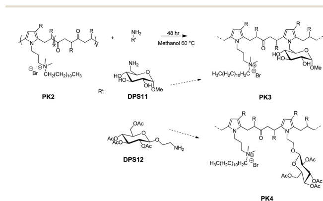
Fig. 12 Schematic representation of the quaternized PKDMP functionalized with DPS11 (PK3) or DPS12 (PK4) via the Paal–Knorr reaction.
