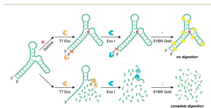
Fig. 1 Schematic illustration of the dual-exonuclease-mediated detecting assay using SYBR Gold as a signal reporter.
