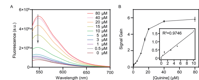
Fig. 5 Performance of the quinine-detecting dual-exonuclease-mediated fluorescence assay in 50% urine. (A) Fluorescence spectra of the samples generated at various quinine concentrations. (B) Calibration curve and linear range derived from the fluorescence spectra. The final concentration of aptamer in reaction solution was 1 \mu\text{M} .
