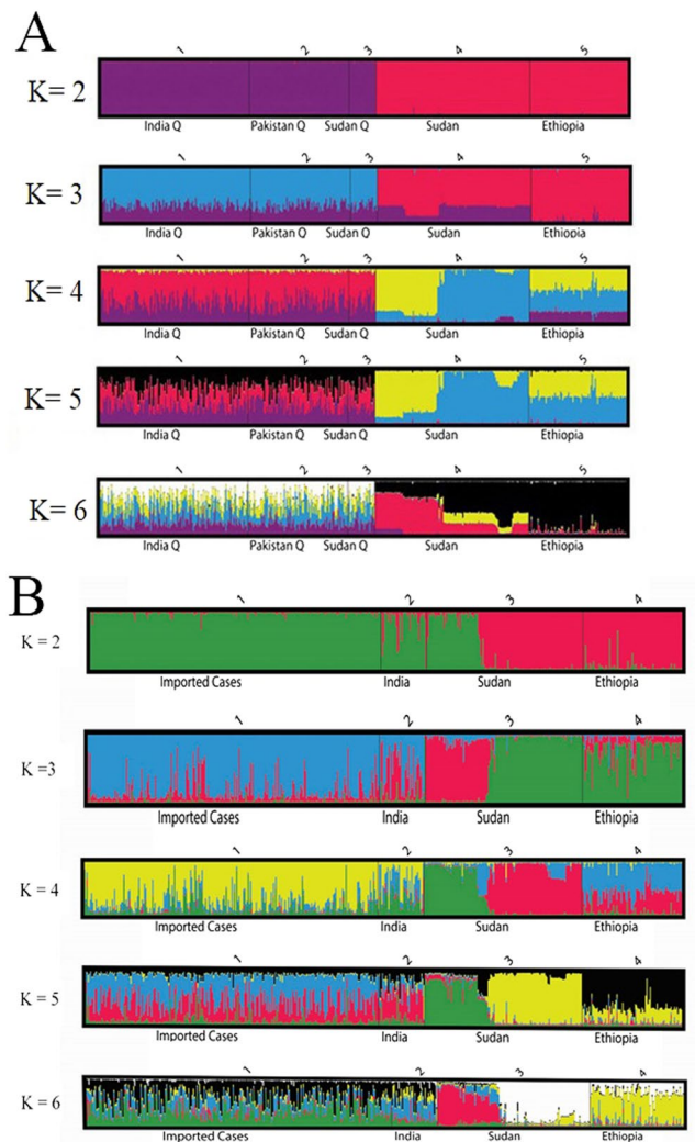
Figure 4. (A) Population Structure. Bar plot illustrating the population structure at K = 2-6 in P. vivax among imported cases in Qatar and parasites from endemic sites in India, Sudan and Ethiopia. Each vertical bar represents an individual sample, and each colour represents one of the K clusters (subpopulations). (B) Population Structure. Bar plot illustrating the population structure at K = 2-6 in P. vivax among imported cases in Qatar and parasites from endemic sites in India, Sudan and Ethiopia. Each vertical bar represents an individual sample, and each colour represents one of the K clusters (subpopulations).
