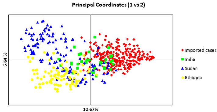
Figure 3. Principal Co-ordinates analysis (PcoA) of P. vivax among imported cases in Qatar and those from endemic sites in India, Sudan and Ethiopia. The amount of variation explained by each axis is shown as a percentage of the overall variation.
