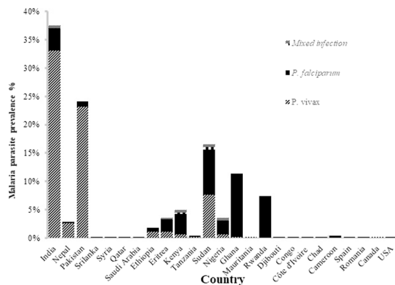
Figure 1. Prevalence of P. vivax , P. falciparum and mixed species infection among imported malaria cases in Qatar between September 2013 and October 2016.
