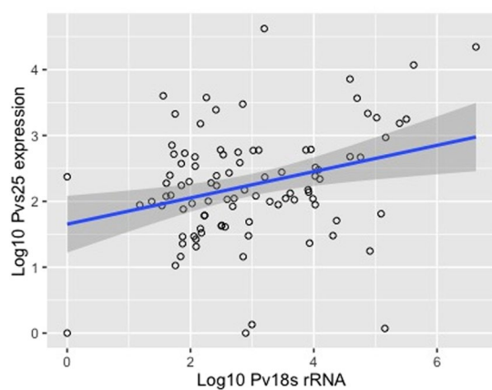
Figure 2. Association between parasite density and gametocyte density among imported P. vivax cases in Qatar (Correlation Coefficient = 0.211, P = 0.04 ).
