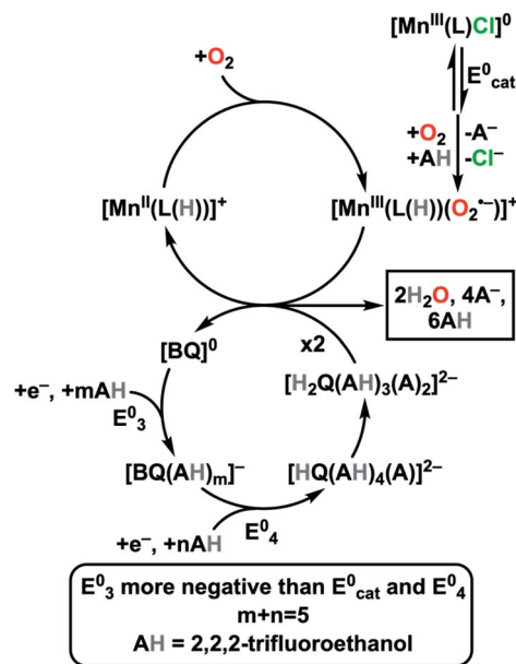
Fig. 5 Proposed potential inversion mechanism for co-electrocatalytic O 2 reduction to water by Mn (t bu dhbpy)Cl 1 and BQ, where AH = TFEOH, m + n = 5 , L = [t bu dhbpy] 2- , and (L(H)) denotes formal protonation of the O atom of the ligand framework.
