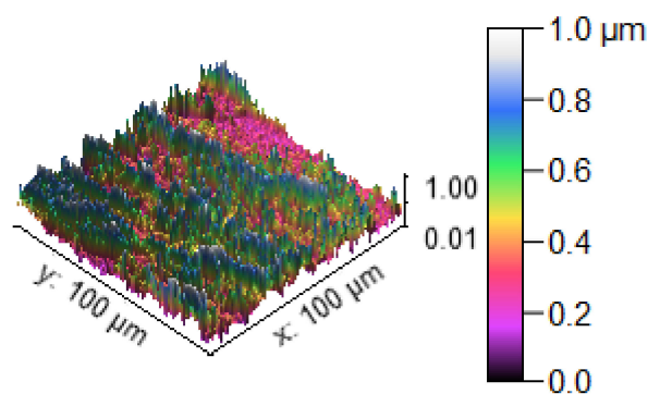
Figure 21. Three dimensional (3D) profilometric image (S-9).
