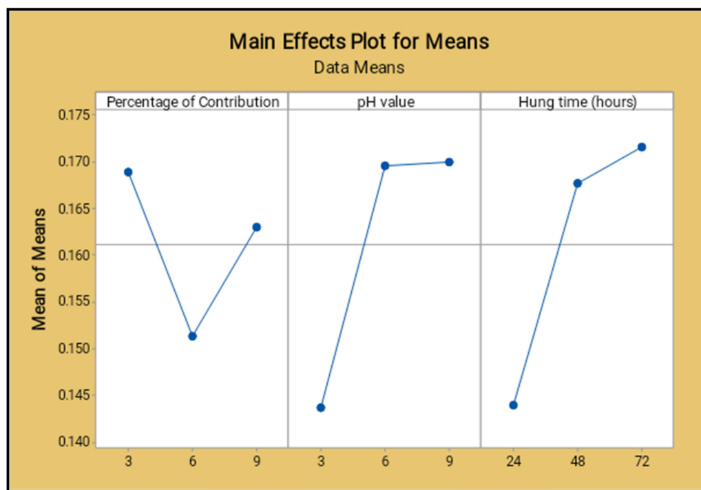
Figure 22. Main effect plot for means (salt spray test).
