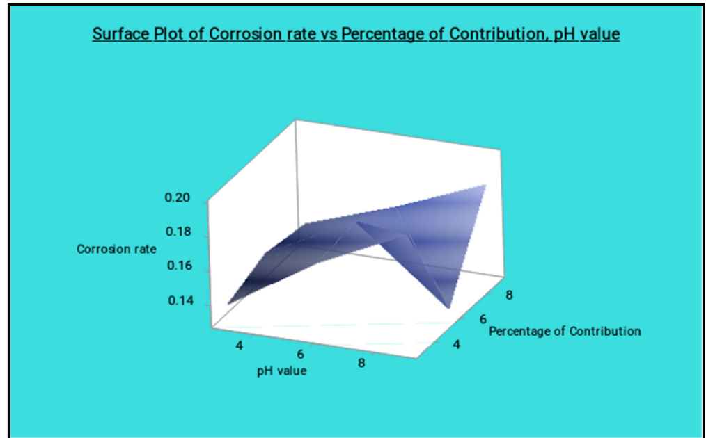
Figure 25. Surface plot of corrosion rate vs. percentage of reinforcement and pH value.
