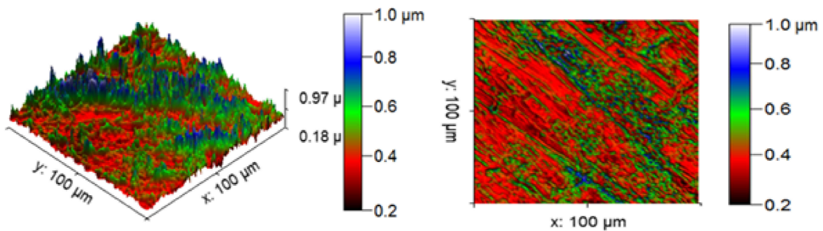
Figure 30. Corrosion test specimen (aximum corrosion).
