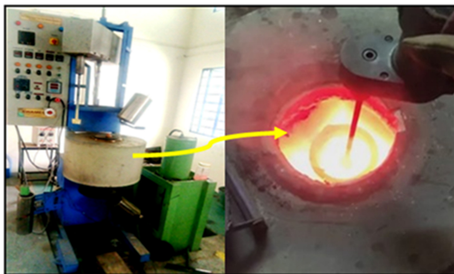
Figure 1. Stir casting process setup.
