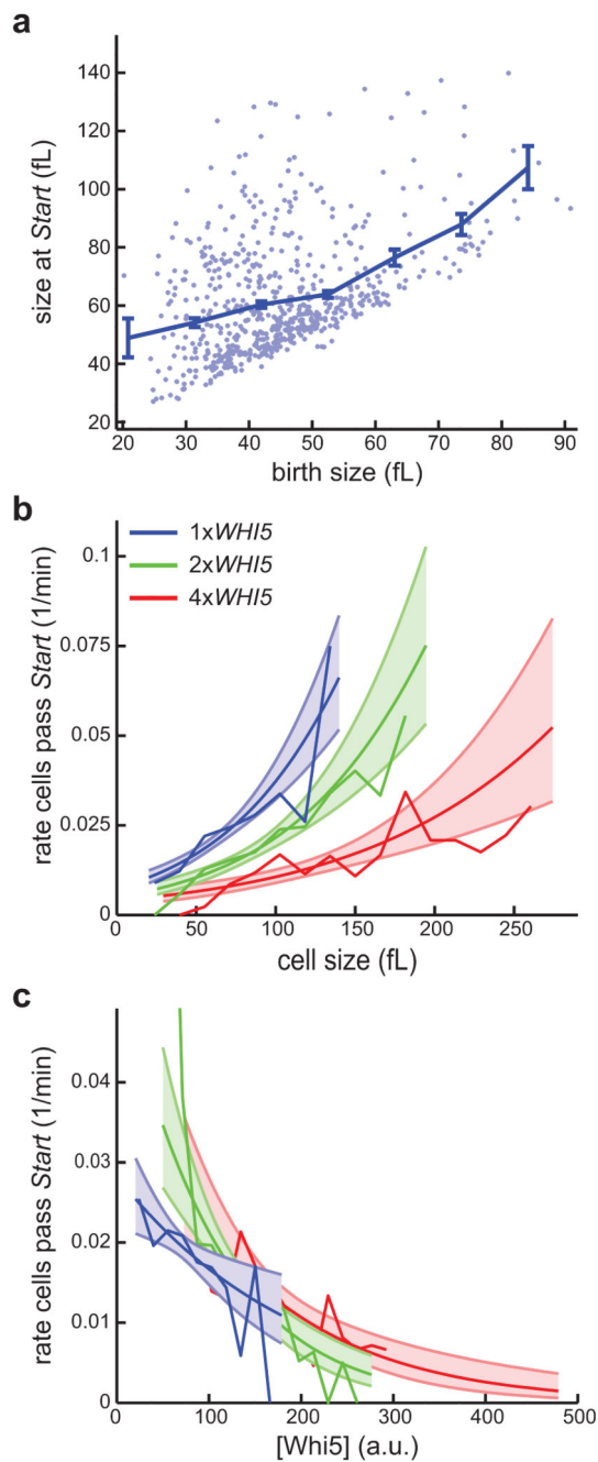
Figure 3. Whi5 concentration determines the rate at which cells progress through Start a , Size at Start , the point of commitment to cell division, as a function of birth size for haploid bck2 daughter cells (n=658). Bars denote mean and standard error. b-c , The rate at which daughter cells progress through Start is shown as a function of cell size ( b ) and Whi5 concentration ( c ) for bck2 haploid cells with one (blue, n=658), two (green, n=310) or four (red, n=142) copies of WHI5-mCitrine . Smooth lines are logistic regressions and the corresponding shaded areas denote 95% confidence intervals. Jagged lines connect means for binned data.
