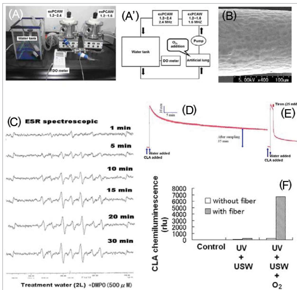
Figure 1. Generation of ROS by SPC processes. (a, a') Water conditioning SPC apparatus. Two exPCAW1.2s (WIPO No: WO10/032765; K2R Inc., Kitakyushu, Japan) connected in tandem (A) and the diagram of water conditioning system (a'). (B) Scanning electron microscopic image of the catalytic fiber which was fabricated by finely coating TiO 2 over alumina layer of aluminum fibers. (C) Detection of DMPO-OH signal with ESR reflecting the generation of HO•. (D) Monitoring of long lasting redox activity in the SPC-processed water using O 2 •- -specific CL probe, CLA. (E) Quenching of CLA-CL by Tiron, a scavenger of O 2 •- . (F) Synergistic impact of UV and USW in generation of O 2 •- . Images were obtained and modified from. 17
