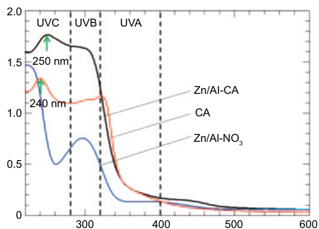
Figure 8 Solid-state absorbance spectra of Zn/Al-NO 3 , organic sunscreen guest cinnamic acid (CA), and the corresponding nanocomposite.
