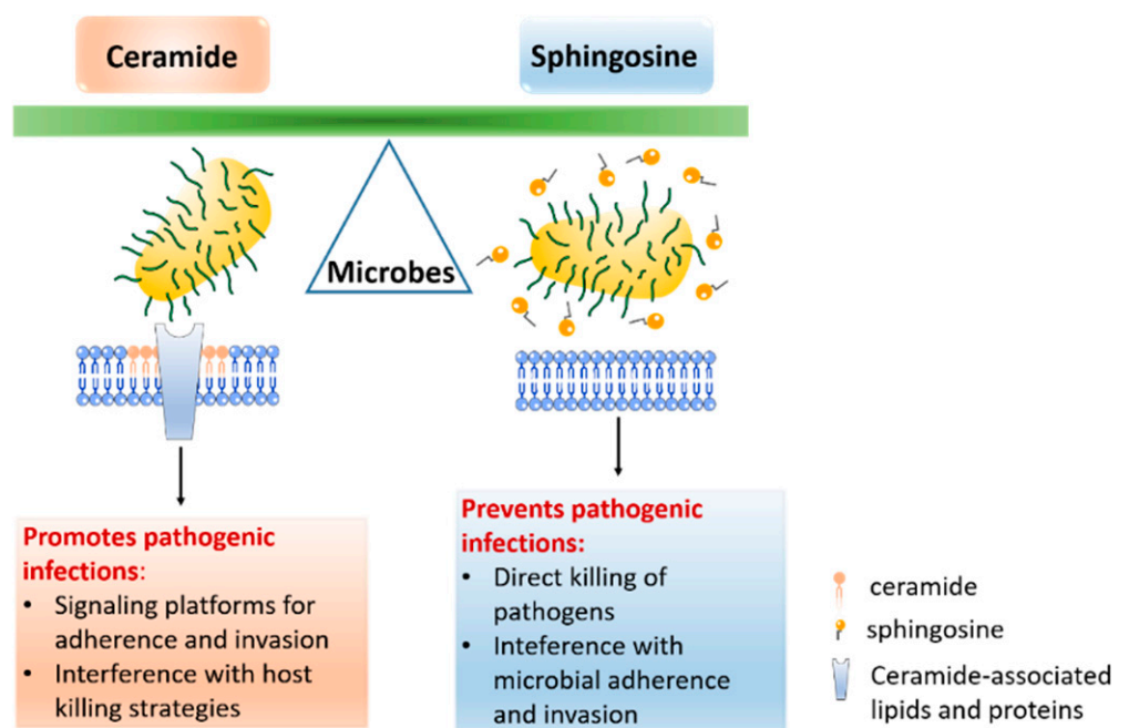
Figure 2. Model illustrating the different effects of ceramide and sphingosine on microbial infections. While sphingosine prevents many bacterial, viral and fungal infections, ceramide often promotes pathogenic infections, by mediating adherence and internalization or by interfering with the killing strategies of the host.
