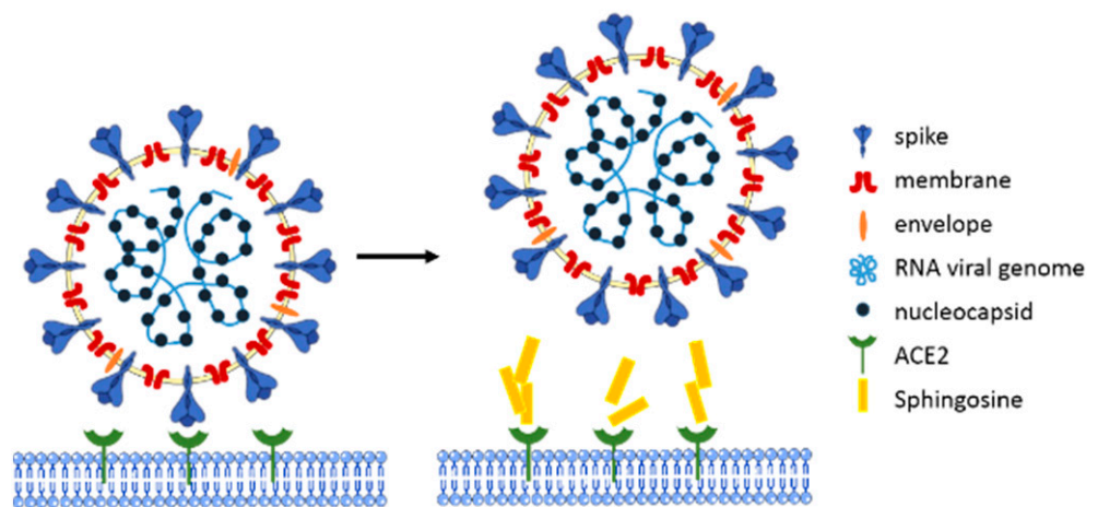
Figure 3. Model of how sphingosine prevents SARS-CoV-2 infection. Exogenous sphingosine application in human nasal or Vero-E6- epithelial cells results in the binding of sphingosine and angiotensin-converting enzyme 2 (ACE2) receptor, which is required for severe acute respiratory syndrome coronavirus-2 (SARS-CoV-2) infection. Sphingosine thereby prevents the recognition and interaction between the spike protein of SARS-CoV-2 and the host's ACE2 receptor and ultimately protects the cells from infection.
