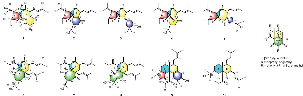
Fig. 1 Structures of compounds 1–10.
