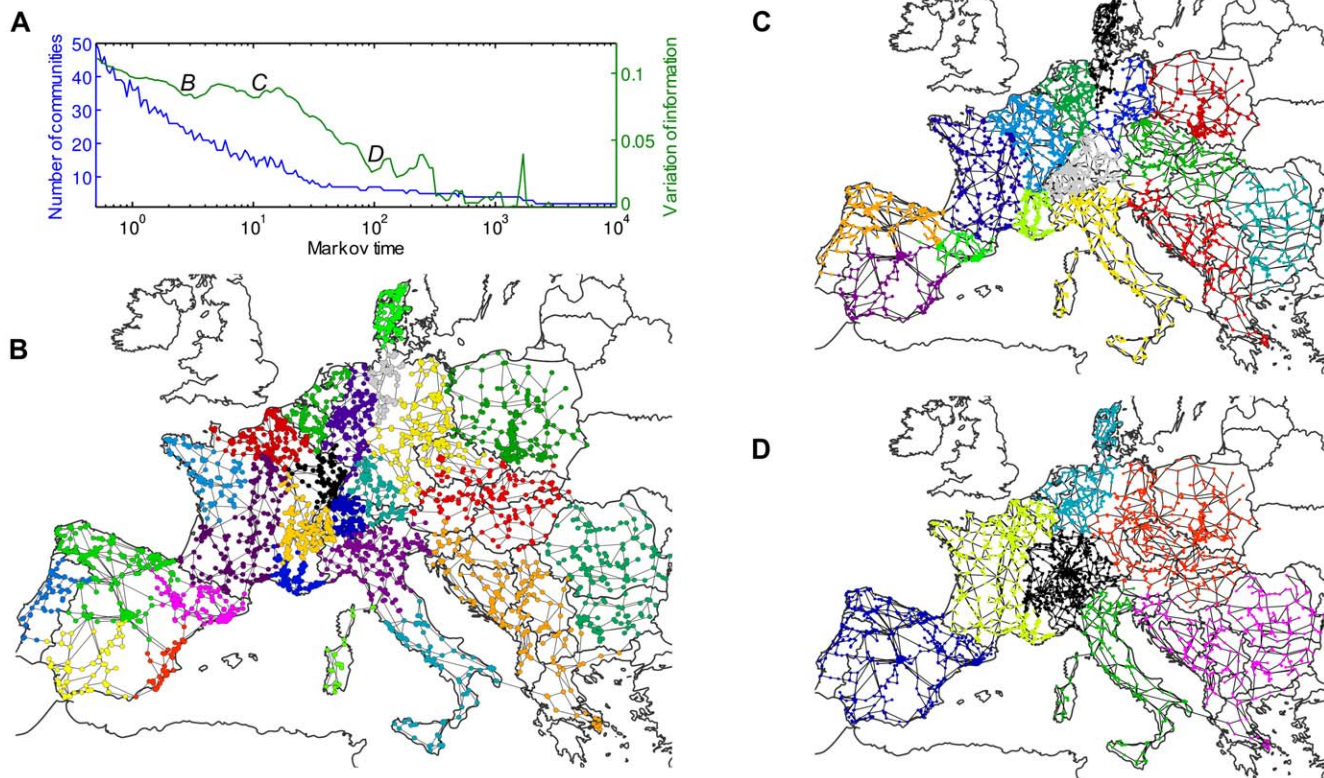
Figure 5. Community structure analysis of the European power grid with stability. A Stability analysis of the community structure of the power grid graph: number of communities found (blue) and average VI (green) vs Markov time. In this case, 1000 initializations of the Louvain algorithm have been used to find the best community and compute the variation of information. B–D Stability finds robust partitions for different Markov times that seem to be related to known structure in the power grid. The partitions shown correspond to Markov times: B t=2.63 (25 communities), C t=11.76 (15 communities) and D t=94.79 (7 communities). doi:10.1371/journal.pone.0032210.g005
