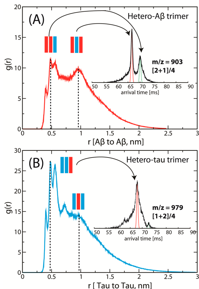
Figure 7. Radial distribution functions g(r) computed for the distances r (nm) (A) between the Ac- A\beta (25–35)-NH 2 monomers within the hetero- A\beta trimer and (B) between the Ac-Tau(273–284)-NH 2 monomers within the hetero-Tau trimer.
