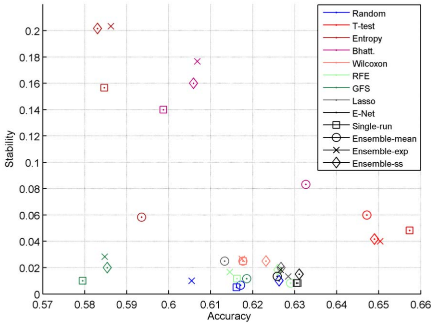
Figure 12. Accuracy/stability trade-off. Accuracy versus stability for each method in the between-datasets setting. We show here the average results over the four datasets. doi:10.1371/journal.pone.0028210.g012
