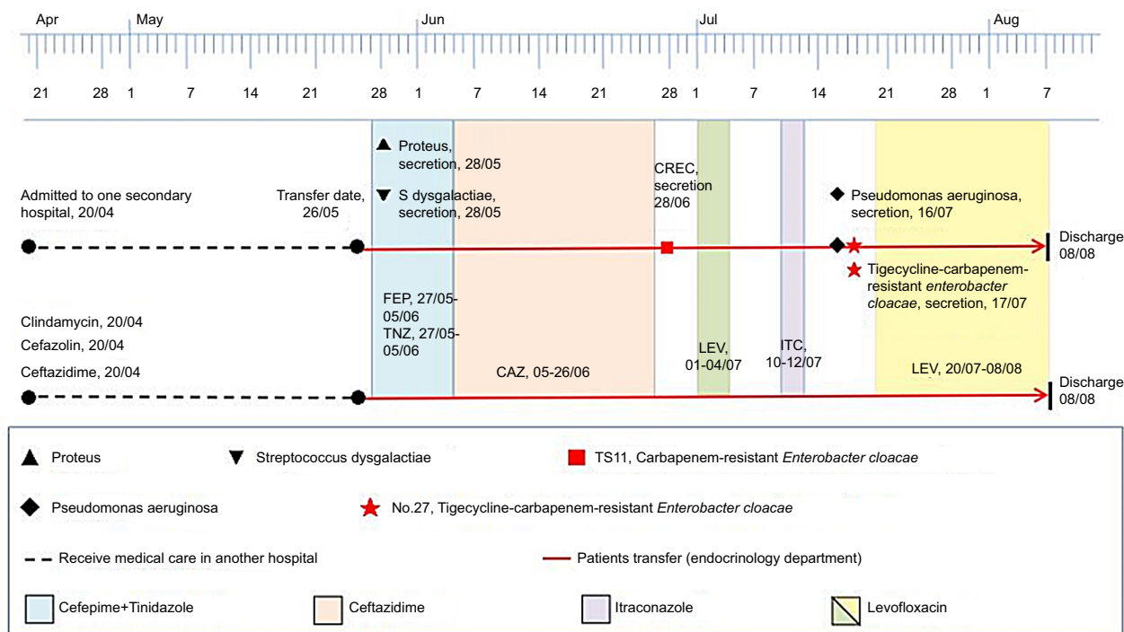
Figure 2 The timeline of the carbapenem-resistant E. cloacae TS.11 and the tigeicycline- and carbapenem-resistant E. cloacae NO.27 isolated from the same patient. Abbreviations: CAZ, ceftazidime; CREC, carbapenem resistant E. cloacae ; FEP, cefepime; ITC, itraconazole; LEV, levofloxacin; TNZ, tinidazole.
