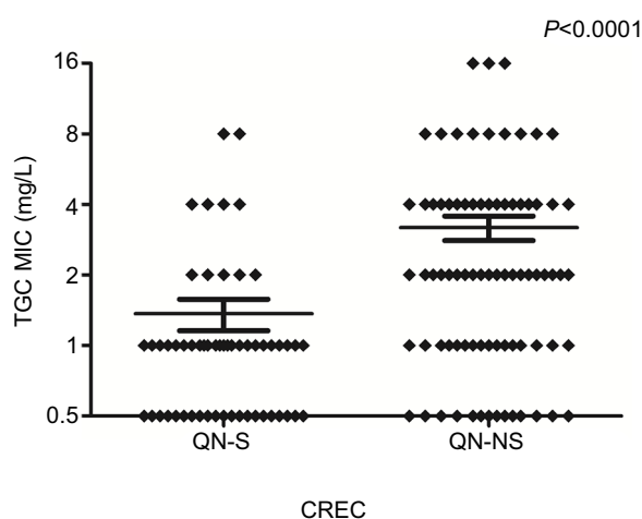
Figure 1 Comparison of tigecycline MICs in QN-S and QN-NS CREC isolates. Abbreviations: CREC, carbapenem resistant E. cloacae ; QN-S, fluoroquinolone-susceptible; QN-NS, fluoroquinolone-non-susceptible; TGC, tigecycline; MIC, minimum inhibitory concentration.
