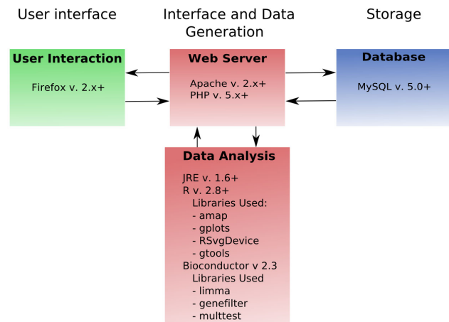
Figure 1 The three layers of EDGE 3 composed of four software components. Communication between the User Interface layer and the Interface and Data Generation layer takes place between the User Interaction component (i.e., the web browser) and Web Server component. Queries from the User Interface layer are routed through the Web Server component to the Storage layer using SQL. Data is returned from the Database component to the Web Server Component and, if necessary, routed to the Data Analysis component where the bioinformatics-based computations take place. If required, the results from the Data Analysis component are returned to the Web Server. In all cases, requested information is sent to the end user and displayed in the User Interaction component (i.e., Firefox web browser) via the Web Server component.
