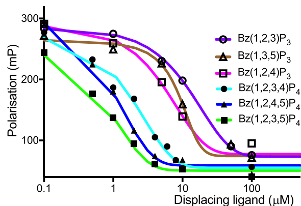
Figure 2. Displacement of 2-FAM-InsP 5 from SHIP2 by benzene phosphates. The experiments used 2 nM 2-FAM-InsP 5 and 1 μM SHIP2. Results shown as mean of triplicate experiments (results with standard deviations given in Table 1).
