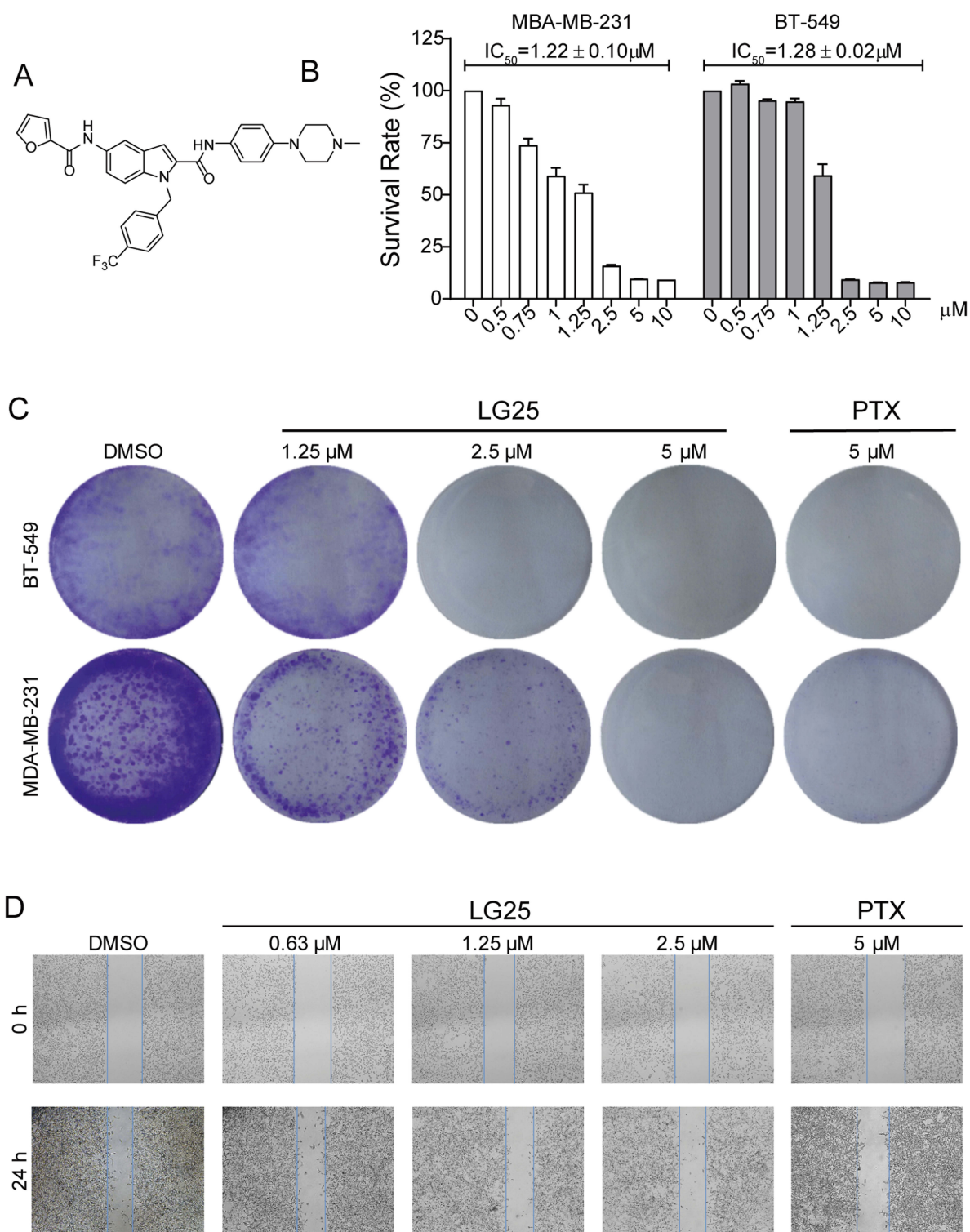
Figure 1 LG25 inhibited cell growth, colony formation, and migration of TNBC cells. (A) The chemical structure of indole-2-carboxamide derivative LG25. (B) Viability of TNBC cells following exposure to LG25. MDA-MB-231 and BT-549 cells were treated with increasing concentrations of LG25 (0.5, 0.75, 1, 1.25, 2.5, 5 or 10 \mu\text{M} ), paclitaxel (PTX, 5 \mu\text{M} ) or vehicle control (DMSO, 1 \mu\text{L} ) for 24 hrs. \text{IC}_{50} values in MBA-MB-231 and BT-549 were obtained using GraphPad Prism 7.0. Data are shown as mean \pm SEM ( n=3 ). (C) Inhibitory effects of LG25 on the colony formation ability of TNBC cells. MDA-MB-231 and BT-549 cells were treated with LG25 at 1.25, 2.5, or 5 \mu\text{M} , paclitaxel at 5 \mu\text{M} , or vehicle control (DMSO, 1 \mu\text{L} ) for 12 hrs. After treatments, cells were cultured for 15 days in drug-free medium. Colonies were stained with crystal violet staining. (D) MDA-MB-231 cells were treated with LG25 at 0.63, 1.25 or 2.5 \mu\text{M} , paclitaxel at 5 \mu\text{M} , or vehicle control (DMSO, 1 \mu\text{L} ) for 24 hrs. The migratory capacity of cells was then assessed. Quantification of the scratch assay is shown in Supplementary Figure S1 .
