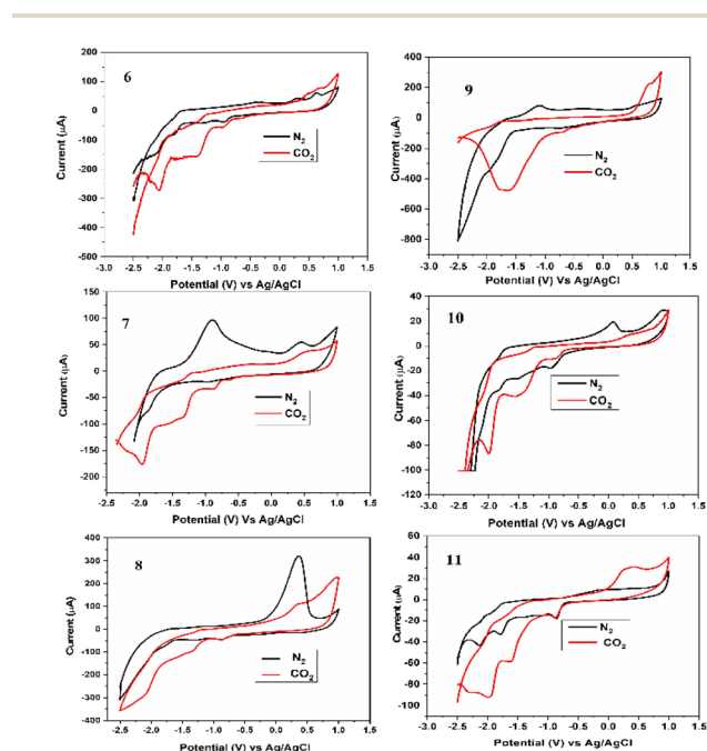
Fig. 3 The cyclic voltammograms of 6–11 under nitrogen (black line) and CO_2 (red line). All experiments were performed at 100\text{ mV s}^{-1} scan rate in DMF and 0.1 M supporting electrolyte (TBAPF 6 ).
