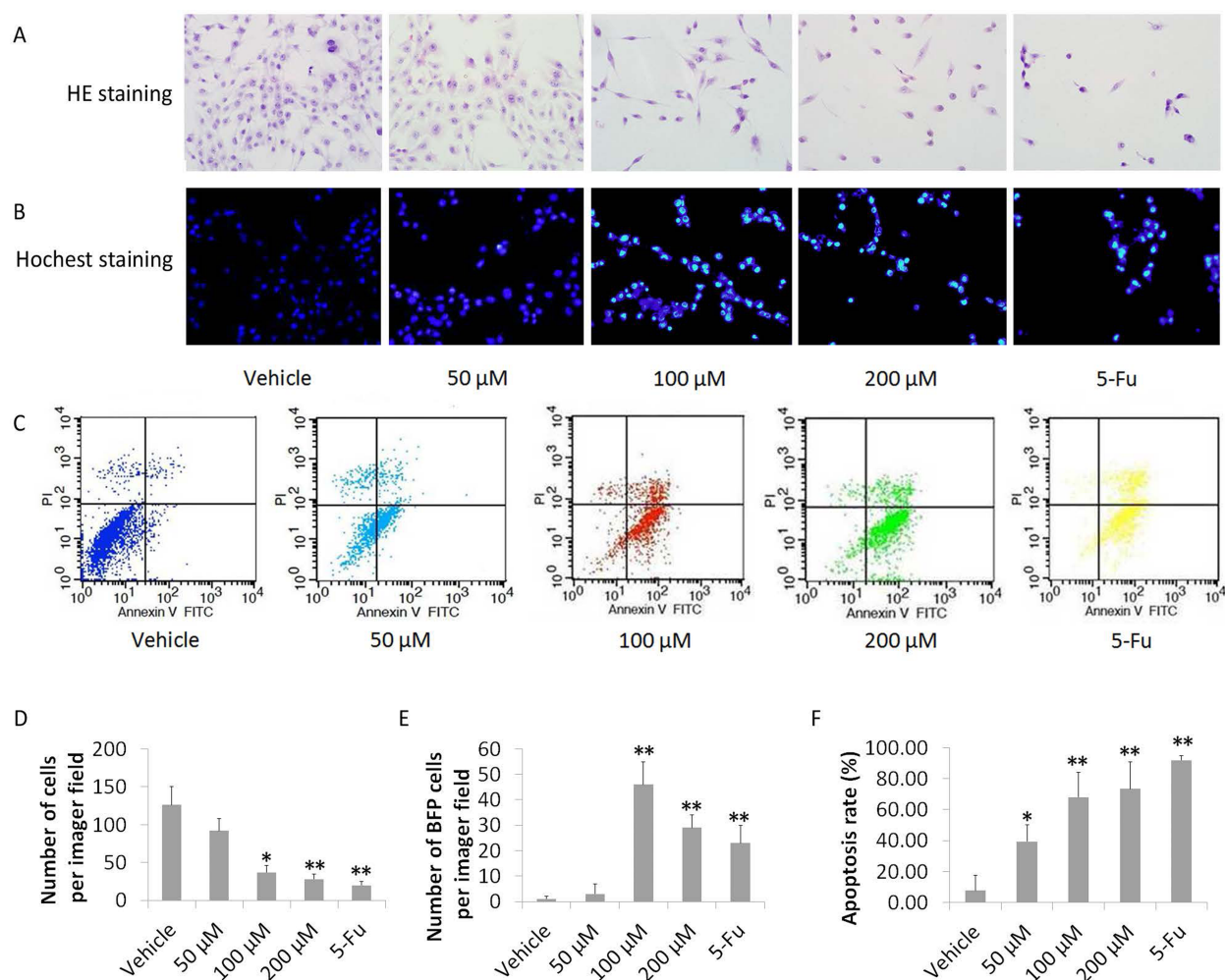
Figure 3. TTF1-NPs induce apoptosis in HepG2 cells. HepG2 cells treated with TTF1-NPs (50, 100, or 200 \mu\text{M} ), 10 \mu\text{M} 5-fluorouracil (5-FU), or DMEM (vehicle) for 48 h were subjected to (A) hematoxylin and eosin staining (400 \times magnification), (B) Hoechst staining (400 \times magnification), and (C) flow cytometry. (D) Quantification of cell numbers from the fields shown in (A) was performed using three independent tests with triplicate samples. (E) Quantification of blue fluorescence-positive (BFP) cell numbers from the fields shown in (B) was performed using three independent tests with triplicate samples. (F) Quantification of cell apoptosis rate (%) was performed based on the results shown in (C) from three independent tests with triplicate samples. The graph shows the corresponding quantified data as mean \pm SD. * p < 0.05 and ** p < 0.01 for the designated treatment versus vehicle.
