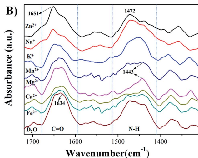
Fig. 5 Infrared absorption spectra of HPEAM-MBA ((A) shows the infrared absorption spectrum of HPEAM-MBA measured in KBr; (B) shows the infrared absorption spectrum of HPEAM-MBA measured in D_2O with or without the metal ions, respectively).
