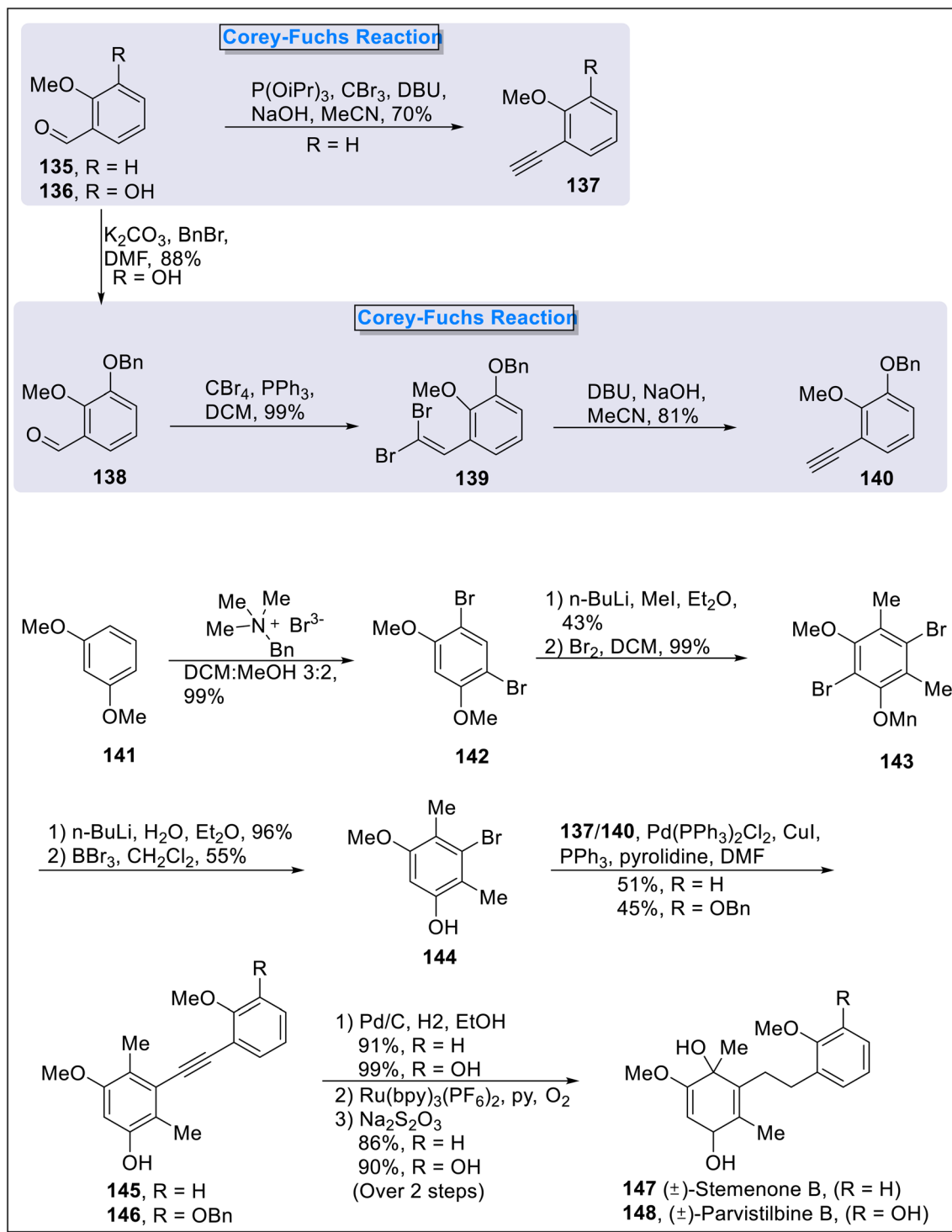
Scheme 13 Total synthesis of (±)-parvistilbine B 148 & (±)-stemenone B 147 by Kozłowski and coworkers.
