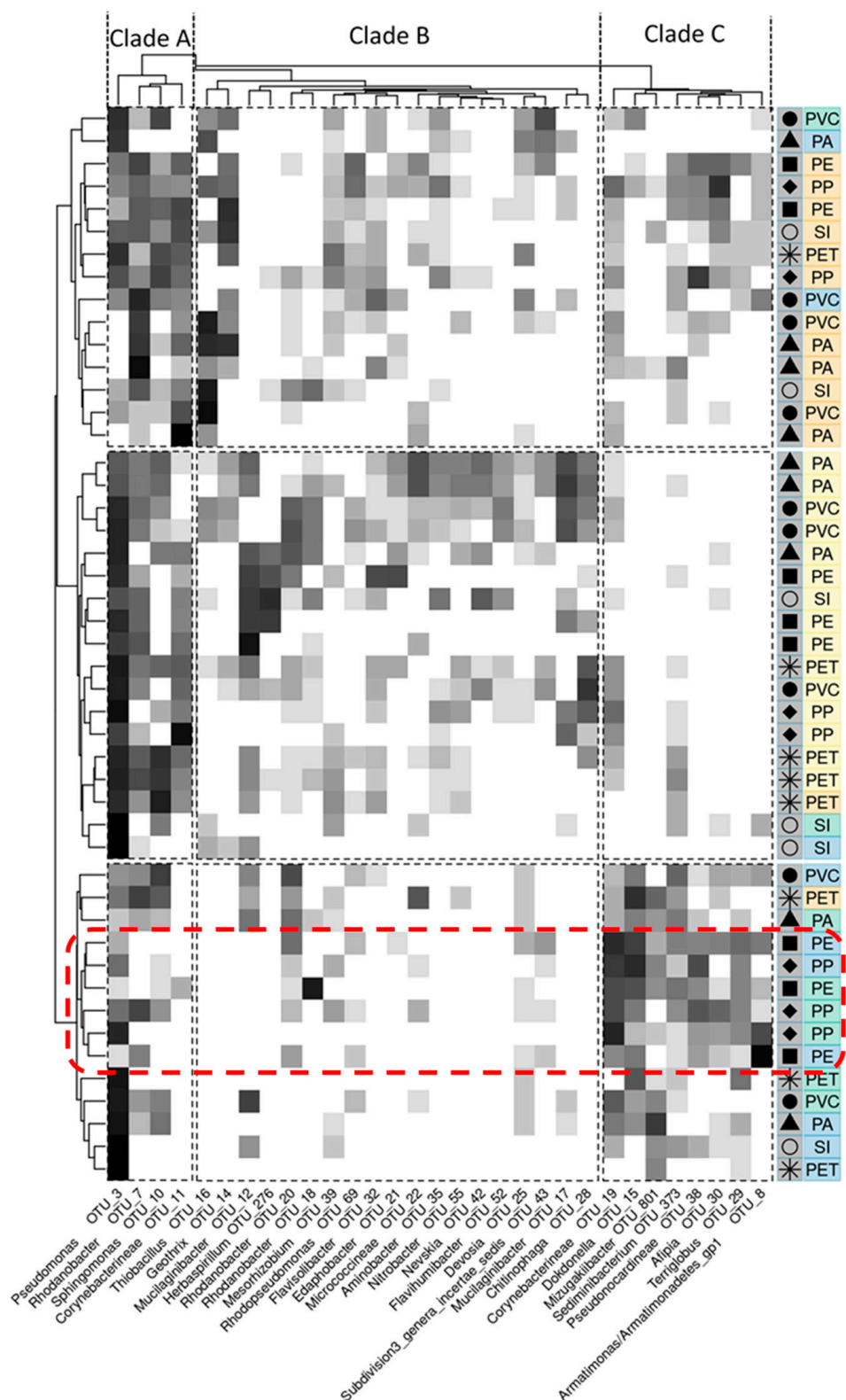
Figure 2. Heatmap based on log-transformed microbial abundances. Colors and icons refer to exposure time and substrate type, as shown in Figure 1. Groups of samples and clades of OTUs are demarked by black dashed lines and defined based on k-means clustering of the euclidean distance between samples. Dendrograms represent euclidean distance clustered via complete linkage. Red box refers to a possible sub-group of > 6-month polyolefins. PA: polyamide; PE: polyethylene; PET: polyethylene terephthalate; PP: polypropylene; PVC: polyvinyl chloride; SI: silica (control).
