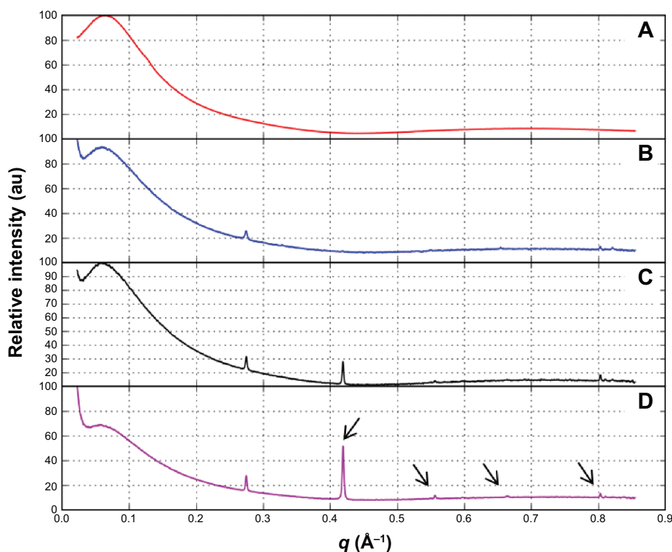
Figure 5 SAXS/WAXS patterns of (A) CDgemiini surfactant; and complexes of NC 2067 with CDgemiini surfactant at three different mole ratios of (B) 1:2, (C) 1:1, and (D) 1:0.5. Arrows show the peaks corresponding to precipitated NC 2067.
