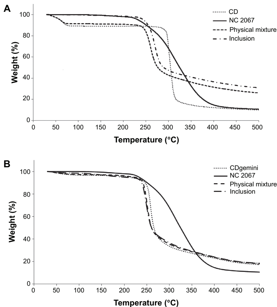
Figure 4 TGA thermograms of (A) CD, NC 2067, physical mixture, and inclusion complex of NC 2067 and CD; and (B) CDgemini surfactant, NC 2067, physical mixture, and inclusion complex of NC 2067 and CDgemini surfactant.
