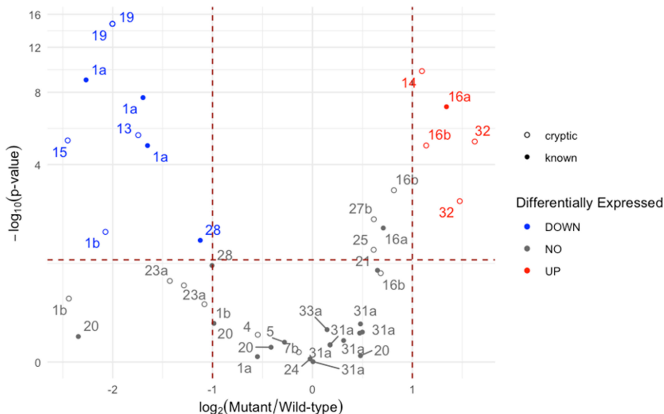
Fig. 5. Volcano plot displaying differentially expressed core BGC genes between the S. scabiei wild-type strain and the \Delta\text{cebR} mutant. Genes belonging to cryptic BGCs are represented by an empty circle, and those from known BGCs by a full one. Colours indicate the differential expression of each core gene in the \Delta\text{cebR} mutant strain relative to the WT: upregulated (red), downregulated (blue), no significant change (grey). The x-axis displays the \text{Log}_2 fold-change (FC) between the mutant and the WT, while the y-axis corresponds to the -\text{Log}_{10} (p-value). Significant expression changes were defined as having a p-value < 0.05 and a \text{Log}_2\text{FC} above or below the given threshold, 1 and -1 respectively ( -1 > \text{Log}_2\text{FC} > 1 ), these limits are represented by dotted red lines on the plot.
