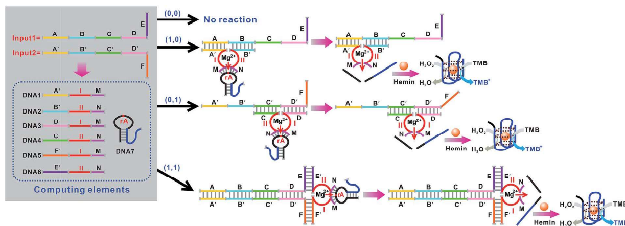
Fig. 7 Schematic representation of the XOR + AND logic gate that consists of the DNAzyme subunits (DNA1–DNA6), the substrate (hairpin DNA7), the caged G-quadruplex sequence in the stem structure of the hairpin is indicated in blue) and the input DNA.
