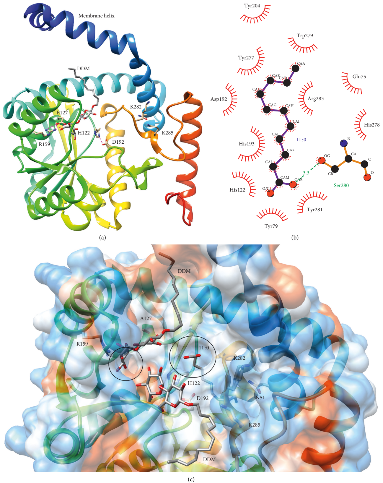
FIGURE 12: LpxM. (a) Ribbon diagram of LpxM (PDB: 5KN7) [86]. Spectrum coloring ends with red at the C-terminus. Interactions between putative catalytic residues are shown. Distances in Ångströms are 2.6 from H122 N \delta to D192 O \delta 1, 2.4 from E127 O \epsilon 1 to R159 N \eta 2 and N \eta 1, and 3.2 from E127 O \epsilon 2 to R159 N \eta 2. (b) Ligplot+ diagram of fatty acid binding to LpxM (PDB: 5KNK) with distance shown in Ångströms [45, 86]. Hydrophobicity surface of LpxM (PDB: 5KNK). Hydrophobicity is shown on an orange-blue scale with blue as the hydrophilic end. The entrances to putative hydrocarbon-ruler channels are circled.
