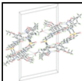
Fig. 3. Crystal packing, viewed along the b axis, of the title complex. The O—H \cdots O, O—H \cdots N and N—H \cdots O interactions are shown as dashed lines.
