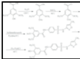
Fig. 1. Synthesis of the title molecule.
