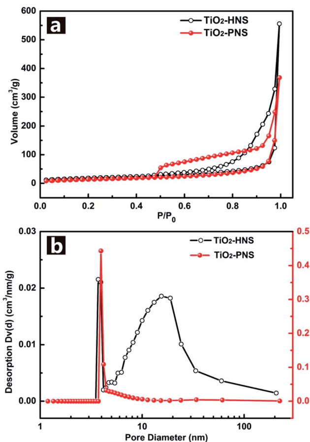
Fig. 3 (a) Nitrogen adsorption/desorption isotherms and (b) Barrett-Joyner-Halenda (BJH) pore-size distribution curves of the TiO 2 -HNSs and TiO 2 -PNSs.
