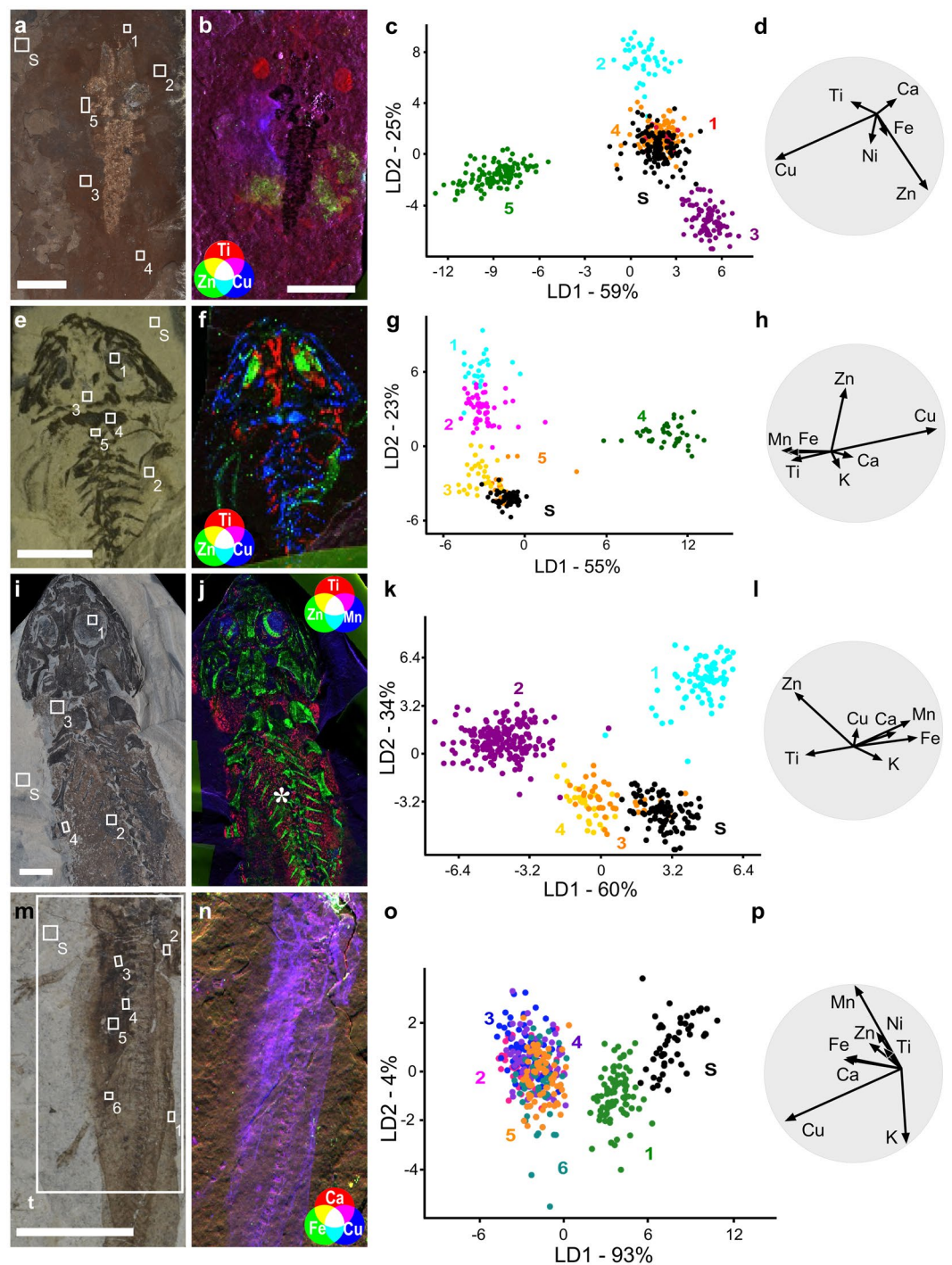
Figure 3. SRS-XRF and LDA analysis of individual fossil specimens. ( a–d ) P. diluvianus (NHML-30271); ( e–h ) B. amplostomus (NHMD-155208); ( i–l ) M. credneri (NHMB-MB-Am.-1187). ( m–p ); Amphibia indet. (CNU-SAL-NN2013002P); ( b,f,j,n ) SRS-XRF tricolor maps of each specimen; maps created using SMAK 1.50 https://www.sams-xrays.com/smak . Asterisks (*) denote internal tissues. ( c,g,k,o ) LDA plot for each specimen; colours and numbers denote different regions of interest; S, sediment. ( d,h,l,p ) biplots showing the most discriminating variables, i.e. those that contribute most to the separation among groups.
