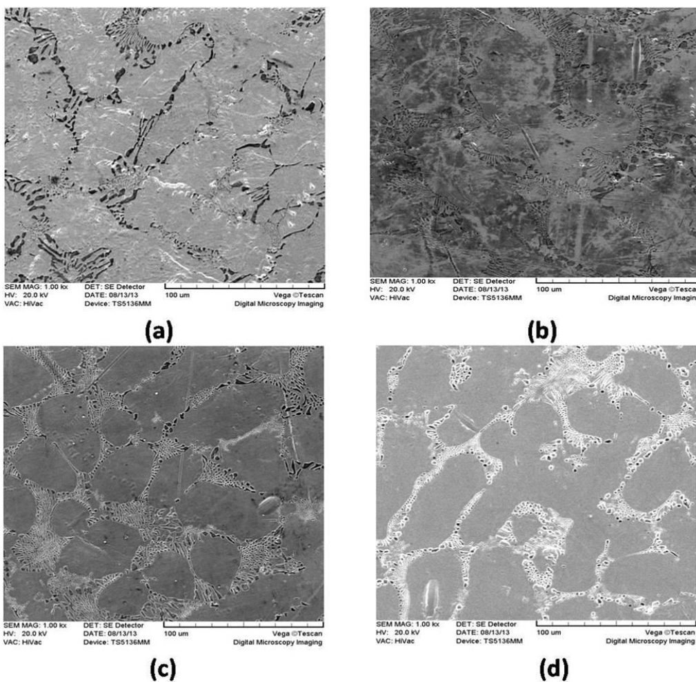
Fig. 4: Scanning electron microscopic (SEM) image of nickel-chromium (Ni-Cr) base alloy after immersion for 5 weeks in artificial saliva at (a) pH=2.5, (b) pH=5, (c) pH=7, and (d) pH=9
