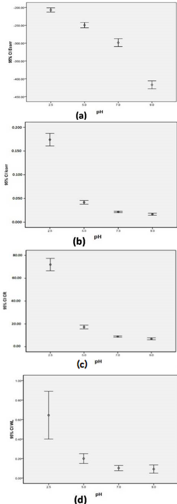
Fig. 2: Error bar of the mean and 95% confidence interval of corrosion parameters measured using two different corrosion tests in artificial saliva. (a) Corrosion potential. (b) Current density. (c) Corrosion rate by the Stern-Geary method. (d) Corrosion rate by weight loss
