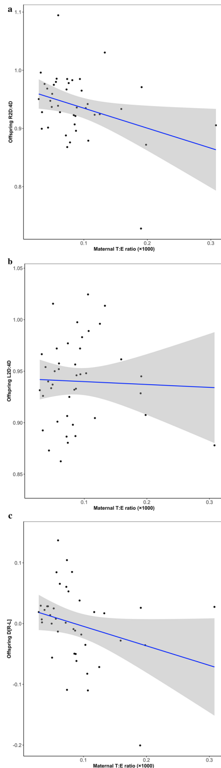
Figure 1. Scatterplots showing the associations between maternal T:E ratio and children's (a) R2D:4D, (b) L2D:4D, and (c) D_{[R-L]} . Raw data (not controlled for covariates) are shown; T:E ratio is multiplied by 1000.
