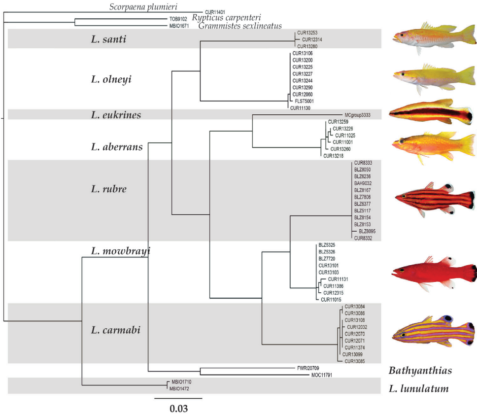
Figure 1. Neighbor-joining tree derived from COI sequences for western Atlantic Liopropoma , the Indo-Pacific L. lunulatum , and related taxa. The tree was rooted on Scorpaena plumieri . Divergence represented by scale bar = 3%. Photographs of L. rubre and L. mowbrayi by James Van Tassel and Ross Robertson.
