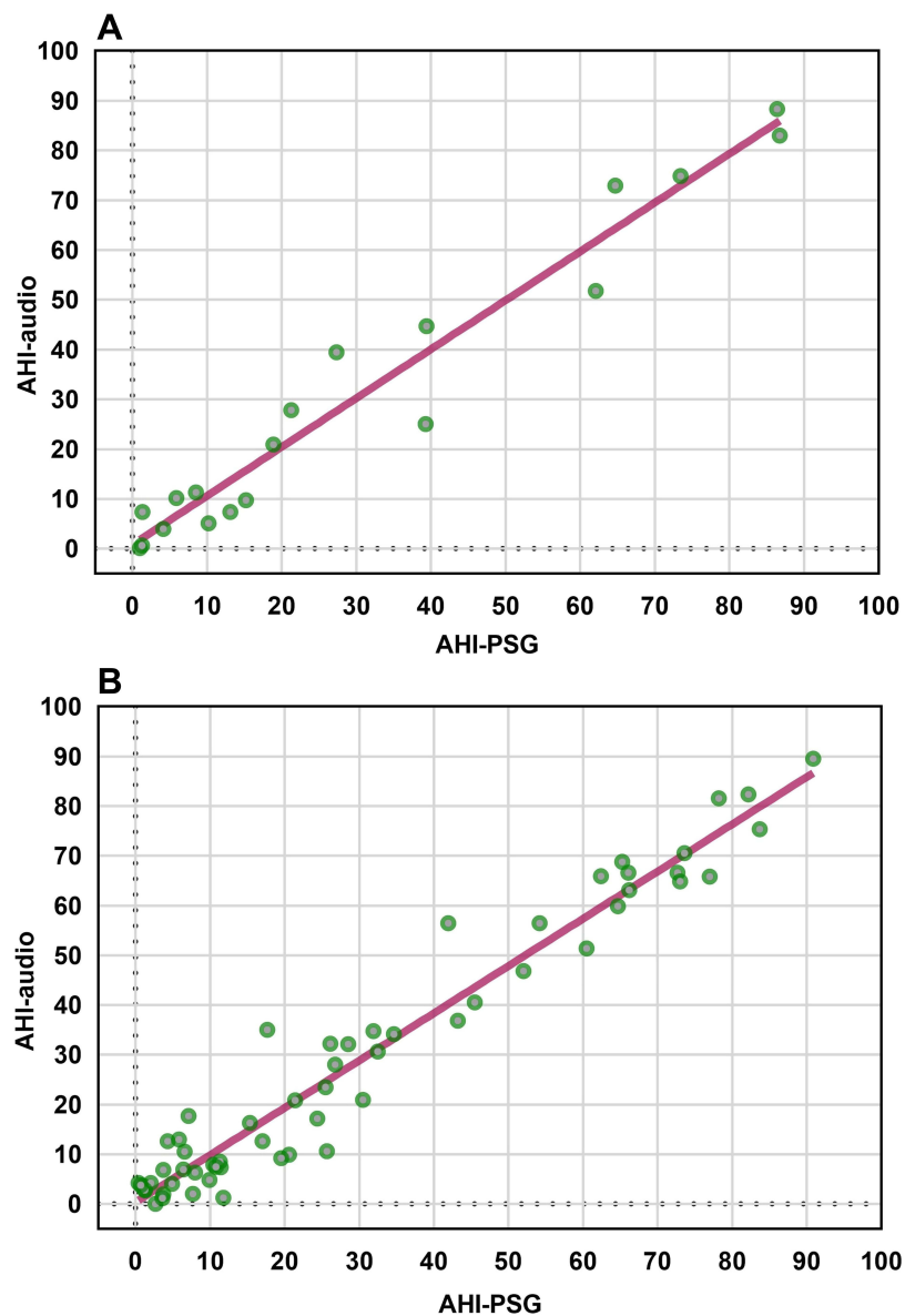
Figure 3 Correlation between AHI-PSG and AHI-audio. Scatter plots of AHI-PSG versus AHI-audio in the validation group ( A ) and test group ( B ). Magenta lines are fit with the two variables ( A ) rho, 0.99, P value<0.01; ( B ), rho, 0.98, P value<0.01).
