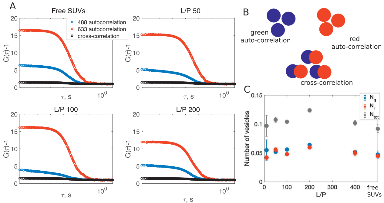
Figure 2. Detecting fusion, fission or vesicle clustering with FCCS. (a) The auto- (green and red) and cross-correlation (black) curves for samples composed of a 1:1 mixture of green and red SUVs with no added protein, and for samples containing SUVs with \alpha -synuclein at L/P 50, 100 and 200. An almost zero amplitude of the cross-correlation curve indicates that none of the samples contains doubly labelled species. (b) Cartoons representing the fluorescent species whose presence is reflected in the auto- and cross-correlation curves. The number of green/red species is inversely proportional to the green/red auto-correlation amplitude, while the number of green-red species is directly proportional to the cross-correlation amplitude. (c) Average number of green and red vesicles \pm SD in the focal volume extracted from the green and red auto-correlation amplitudes corrected for the contribution from the residual free dye (higher amount of residual free dye for green-fluorescent lipids than for red fluorescent lipids). The total number of vesicles \pm SD was calculated as the sum of N_g and N_r . The fact that the average number of vesicles in the focal volume is lower than 1 means that SUVs are present in the focus for only a fraction of the measurement time.
