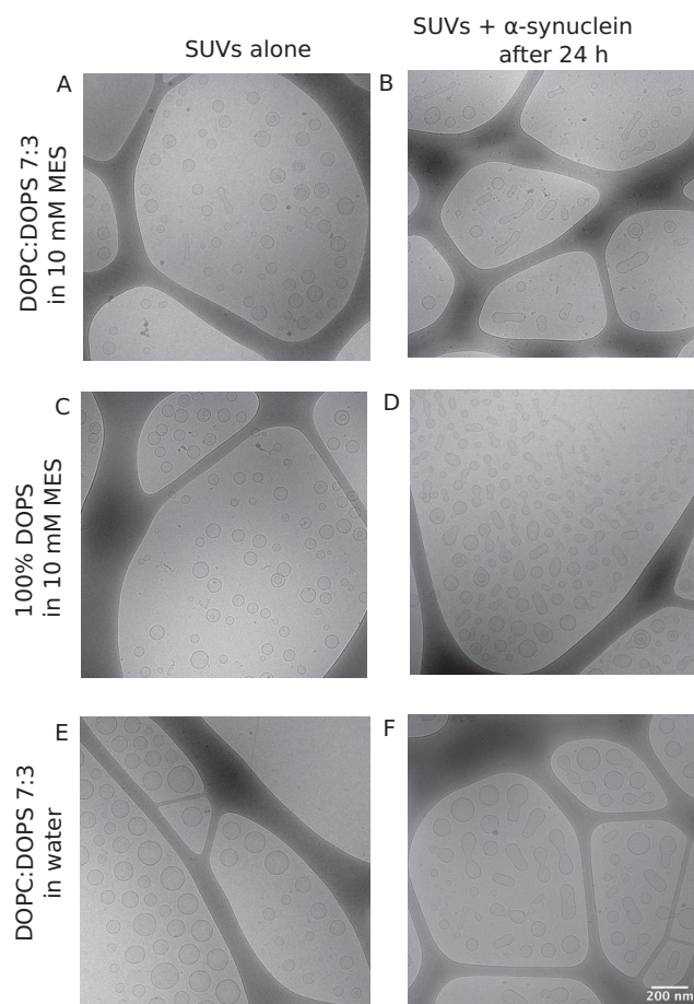
Figure 1. \alpha -Synuclein induces deformation of SUVs. Cryo -TEM images of SUVs without and with \alpha -synuclein at L/P 200. (a,b) DOPC:DOPS 7:3 SUVs in 10 mM MES buffer pH 5.5. (c,d) 100% DOPS SUVs in 10 mM MES buffer pH 5.5. (e,f) DOPC:DOPS 7:3 SUVs in pure water. The scale bar is shown in panel f and is the same for all images.
