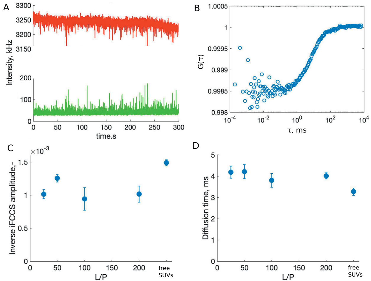
Figure 3. Determining the change in volume of the vesicles upon \alpha -synuclein binding with iFCCS. (a) Green-labelled vesicles (0.5% Oregon Green 488 DHPE) give rise to a positive signal in the green intensity trace (bottom) and to a negative signal in the red intensity trace (top) due to displacement of red fluorescent dye from the detection volume. (b) An example of an anti-correlation curve. The fluctuations of the signals from the green and red channels are cross-correlated giving rise to an anti-correlation function whose amplitude is proportional to the volume of the vesicles. The iFCCS curves for all samples are shown in Supplementary Fig. 2. (c) The inverse of the amplitude of the iFCCS function \pm SD as a function of L/P ratio. (d) Diffusion time of the vesicle \pm SD as a function of L/P ratio extracted from the auto-correlation curves in the green channel.
