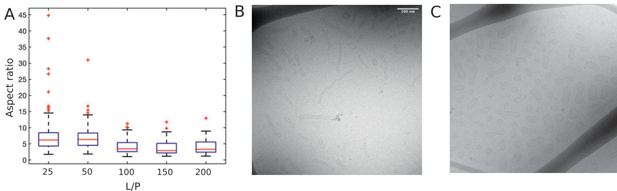
Figure 4. The extent of SUV deformation as a function of the lipid-to-protein ratio (L/P). (a) Box-whiskers plot of the aspect ratio of DOPC:DOPS 7:3 SUVs with \alpha -synuclein imaged with cryo-TEM as a function L/P. The aspect ratio was calculated as the ratio between the long and the short axis of the vesicle. For each L/P, 100 vesicles were analysed. (b) Cryo-TEM image of DOPC:DOPS 7:3 SUVs with \alpha -synuclein at L/P 50. (c) Cryo-TEM image of DOPC:DOPS 7:3 SUVs with \alpha -synuclein at L/P 200. The scale bar for both images is the same and is shown in panel b.
