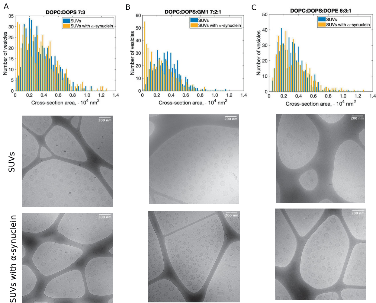
Figure 5. Cross-section area analysis of SUVs without and with \alpha -synuclein imaged with cryo -TEM. (a,b,c) Histogram of cross-section areas of SUVs composed of DOPC:DOPS 7:3, DOPC:DOPS:GM1 7:2:1 and DOPC:DOPS:DOPE 6:3:1, respectively. Examples of the analysed images are shown below the histograms. The samples containing SUVs and \alpha -synuclein (L/P 200) were imaged 24 h after the addition of the protein. For each sample, 550 vesicles from different images were analysed.
